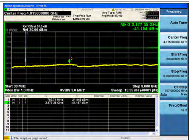
Band14 / 10MHz / High CH / 64QAM
