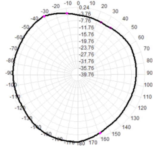
Total(H-XY), Max=0.24dBi, CirD=6.35
