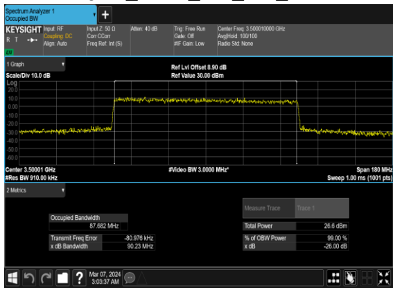
N77(90M)_CP-OFDM_64 QAM_Outer_Full_Mid_CH
