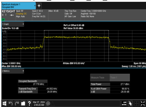
N77(30M)_CP-OFDM_16 QAM_Outer_Full_Mid_CH
