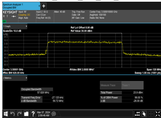
N77(60M)_CP-OFDM_256 QAM_Outer_Full_Mid_CH
