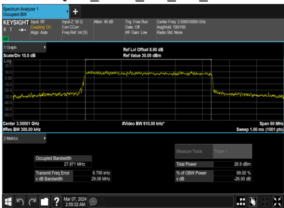
N77(30M)_CP-OFDM_64 QAM_Outer_Full_Mid_CH
