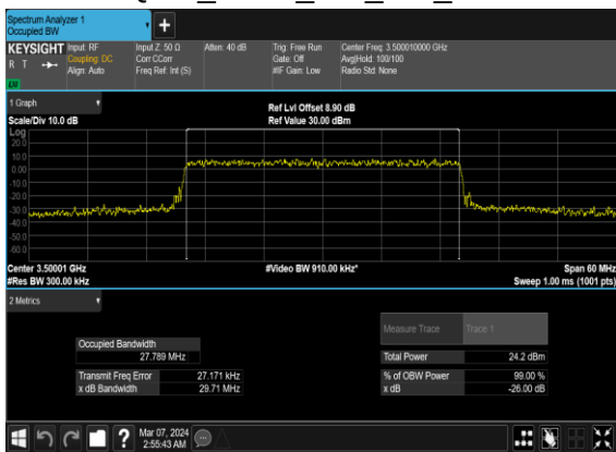
N77(30M)_CP-OFDM_256 QAM_Outer_Full_Mid_CH
