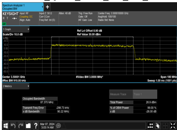
N77(90M)_CP- OFDM_QPSK_Outer_Full_Mid_CH
