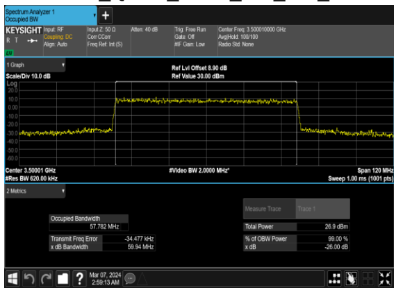
N77(60M)_CP- OFDM_QPSK_Outer_Full_Mid_CH
