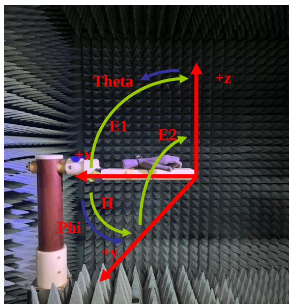
Figure 4: Geometry for SM-L300 for Radiation patterns.
