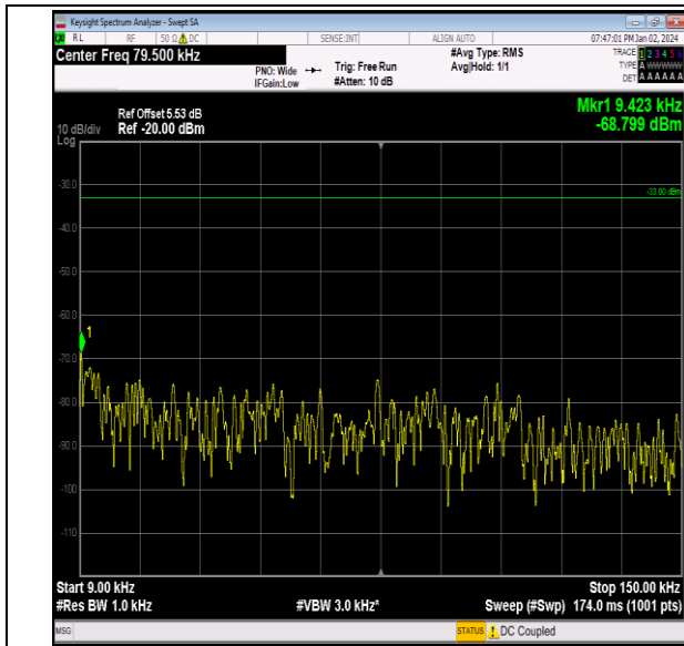
Band26_1.4MHz_16QAM_26740_1RB#0_0.009~0.15_0.0 09~0.15
