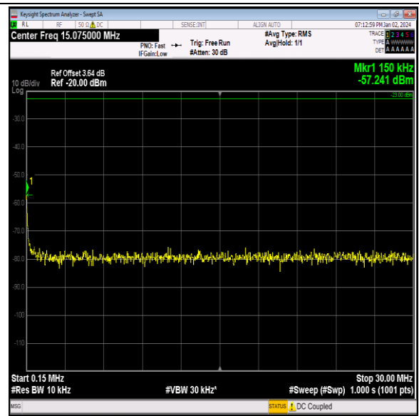
Band13_5MHz_16QAM_23230_1RB#0_0.15~30_0.15~30
