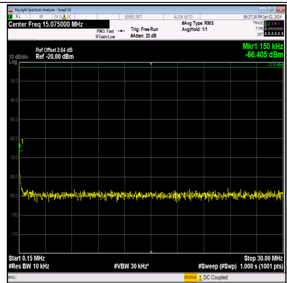
Band26_5MHz_QPSK_26715_1RB#0_0.15~30_0.15~30
