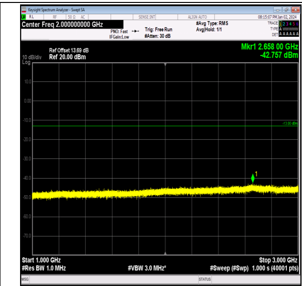
Band26_3MHz_16QAM_26740_1RB#0_1000~3000_1000 ~3000
