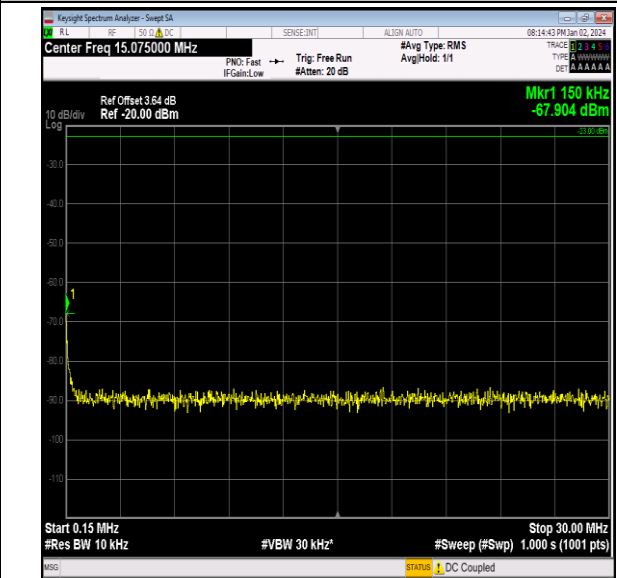
Band26_3MHz_16QAM_26740_1RB#0_0.15~30_0.15~30
