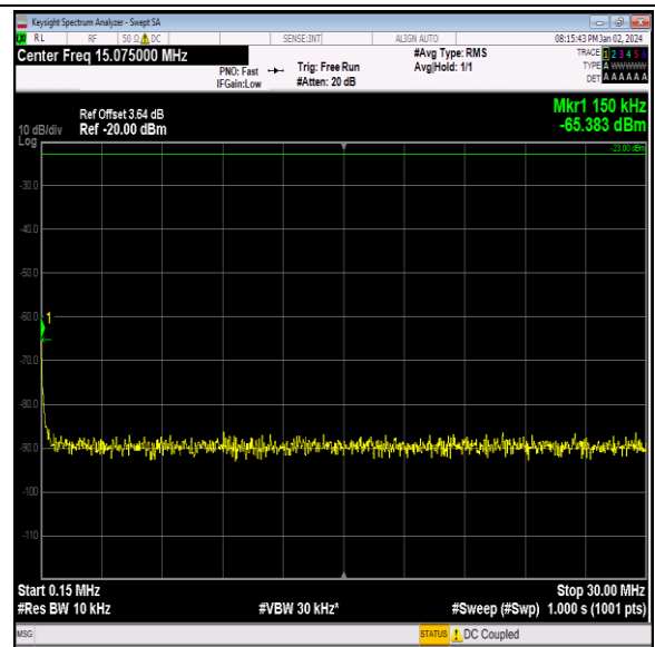
Band26_3MHz_QPSK_26775_1RB#0_0.15~30_0.15~30
