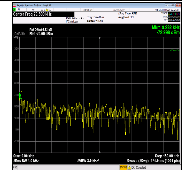
Band26_3MHz_QPSK_26740_1RB#0_0.009~0.15_0.009~0.15
