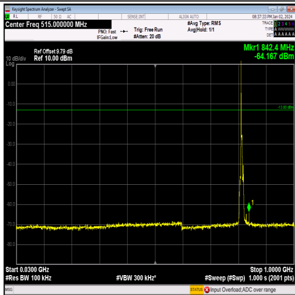
Band26_5MHz_QPSK_26715_1RB#0_30~1000_30~1000
