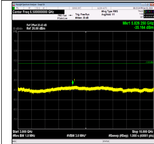
Band26_3MHz_16QAM_26740_1RB#0_3000~10000_300 0~10000
