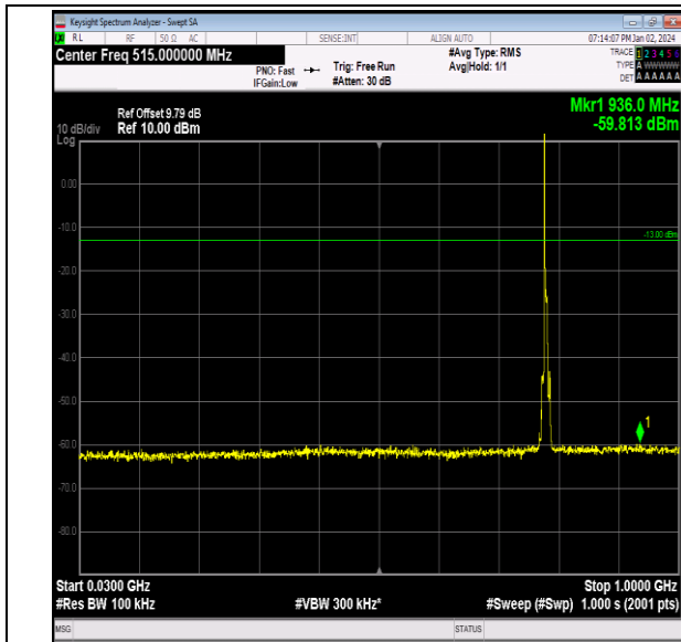
Band13_5MHz_QPSK_23255_1RB#0_30~1000_30~1000
