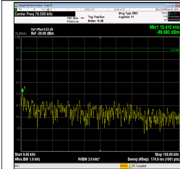
Band26_3MHz_16QAM_26740_1RB#0_0.009~0.15_0.009 ~0.15
