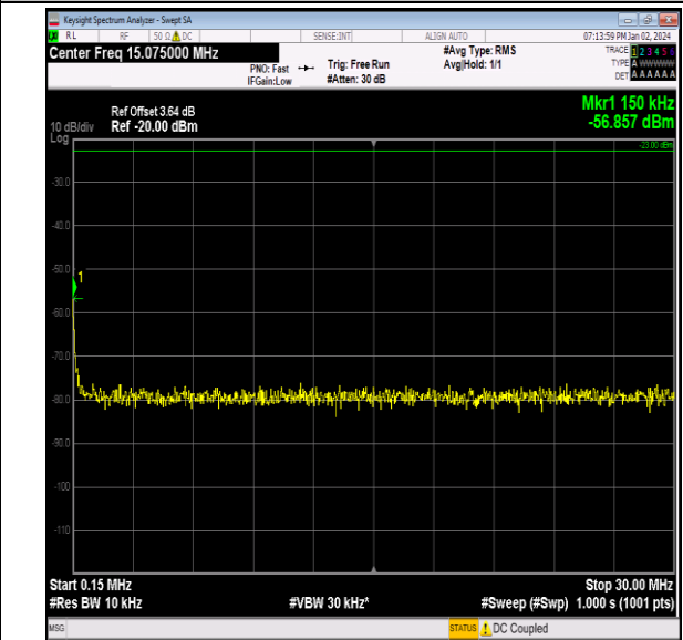
Band13_5MHz_QPSK_23255_1RB#0_0.15~30_0.15~30
