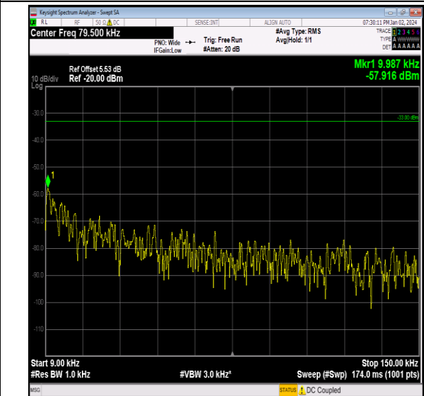
Band13_10MHz_16QAM_23230_1RB#0_0.009~0.15_0.00 9~0.15
