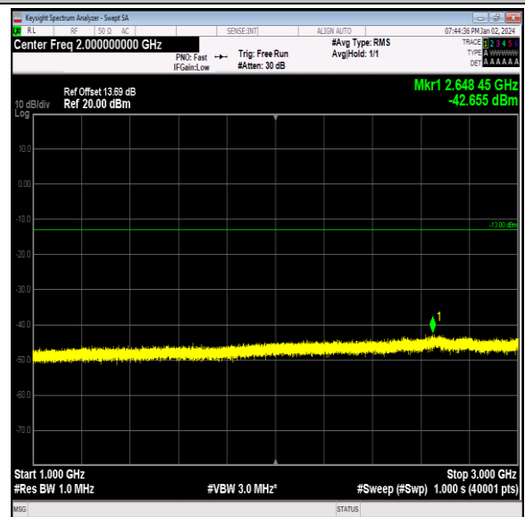
Band26_1.4MHz_QPSK_26697_1RB#0_1000~3000_1000 ~3000
