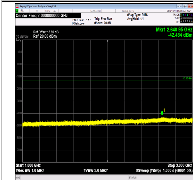
Band26_3MHz_QPSK_26740_1RB#0_1000~3000_1000~3000
