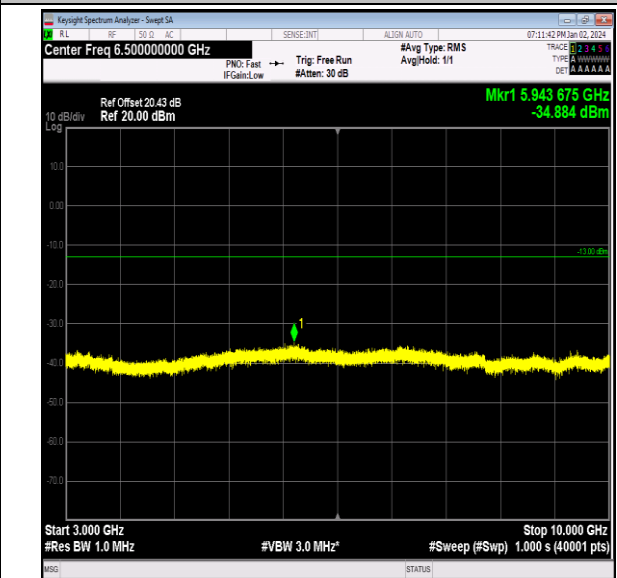
Band13_5MHz_16QAM_23205_1RB#0_3000~10000_3000 0~10000
