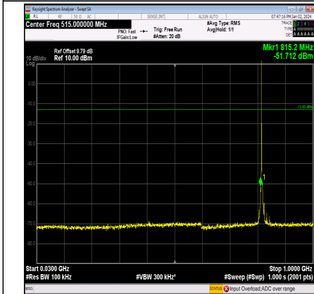
Band26_1.4MHz_16QAM_26740_1RB#0_30~1000_30~1 000
