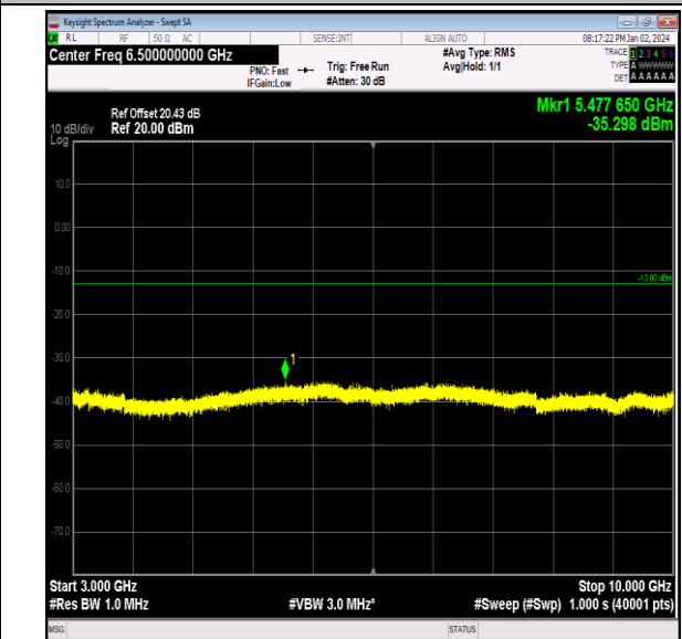
Band26_3MHz_16QAM_26775_1RB#0_3000~10000_3000 0~10000
