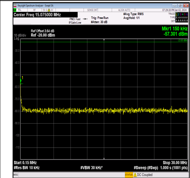
Band13_10MHz_QPSK_23230_1RB#0_0.15~30_0.15~30
