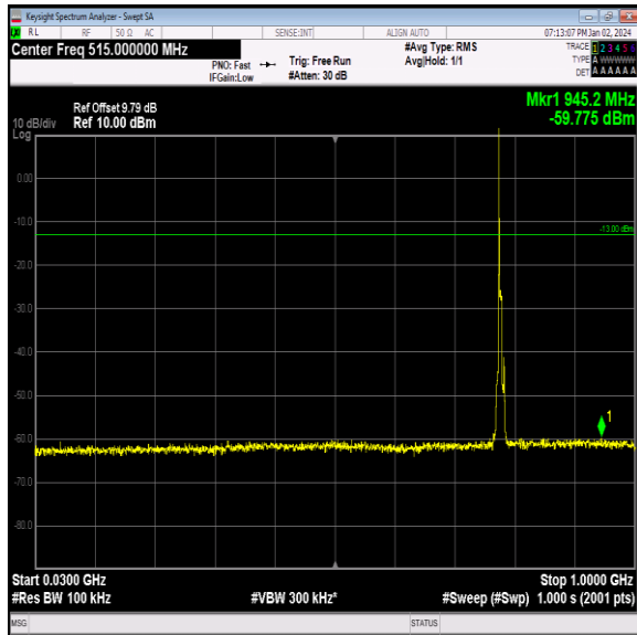
Band13_5MHz_16QAM_23230_1RB#0_30~1000_30~100 0
