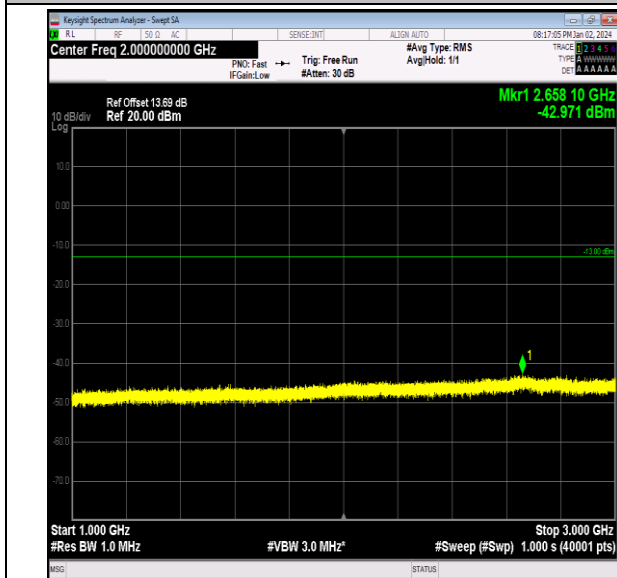
Band26_3MHz_16QAM_26775_1RB#0_1000~3000_1000 ~3000
