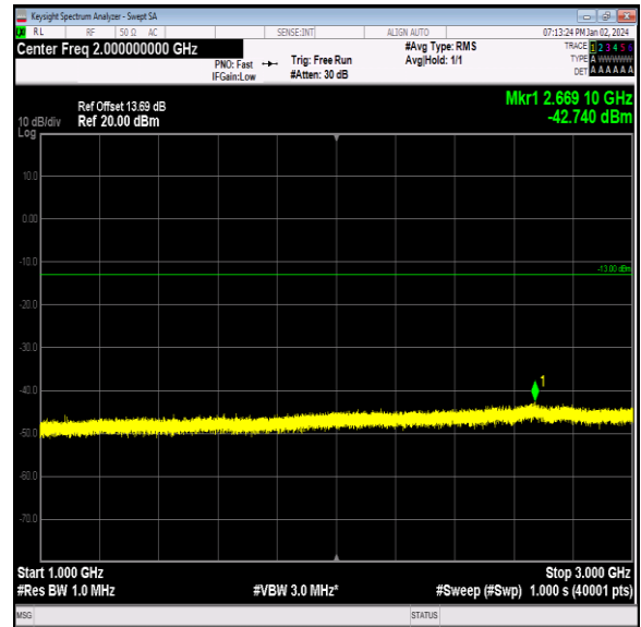
Band13_5MHz_16QAM_23230_1RB#0_1000~3000_1000 ~3000
