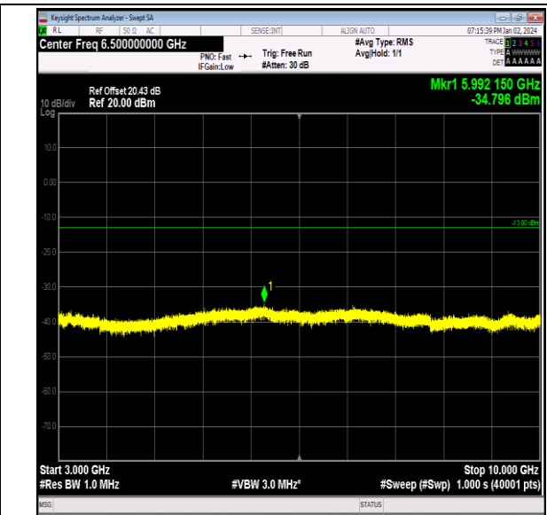
Band13_5MHz_16QAM_23255_1RB#0_3000~10000_300 0~10000
