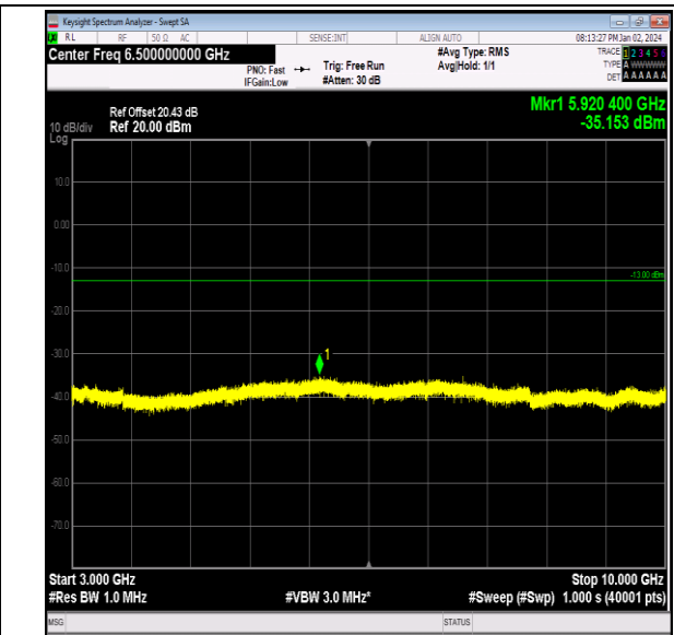
Band26_3MHz_16QAM_26705_1RB#0_3000~10000_300 0~10000
