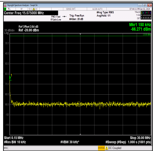
Band26_1.4MHz_QPSK_26697_1RB#0_0.15~30_0.15~30
