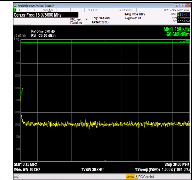
Band26_3MHz_QPSK_26705_1RB#0_0.15~30_0.15~30
