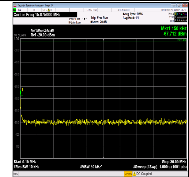
Band26_1.4MHz_QPSK_26783_1RB#0_0.15~30_0.15~30
