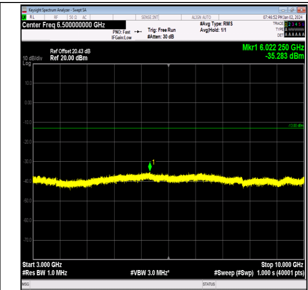
Band26_1.4MHz_QPSK_26740_1RB#0_3000~10000_300 0~10000
