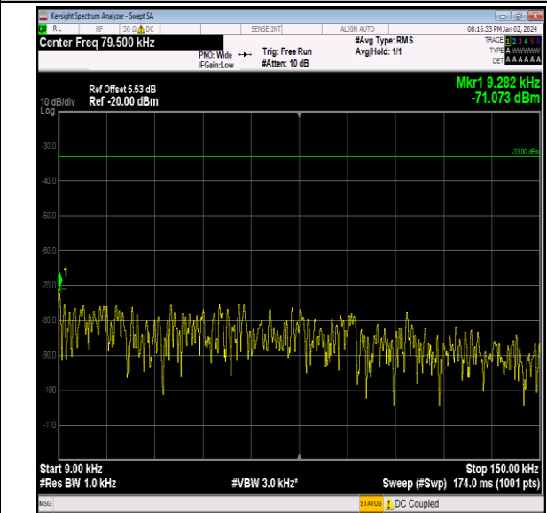
Band26_3MHz_16QAM_26775_1RB#0_0.009~0.15_0.009 ~0.15
