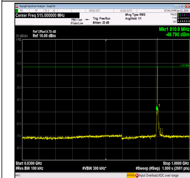
Band26_1.4MHz_QPSK_26697_1RB#0_30~1000_30~100 0
