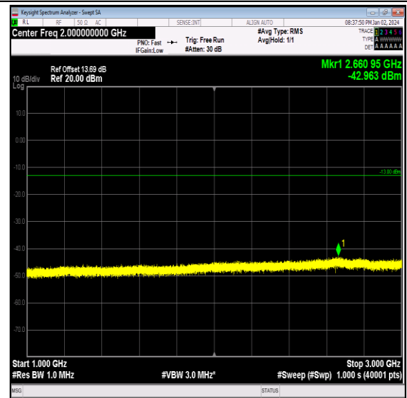
Band26_5MHz_QPSK_26715_1RB#0_1000~3000_1000~3000
