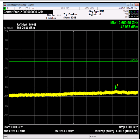
Band26_3MHz_QPSK_26775_1RB#0_1000~3000_1000~3000
