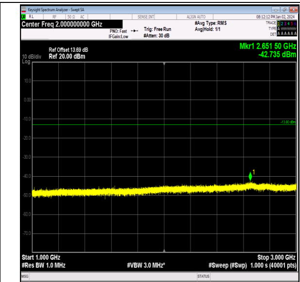
Band26_3MHz_QPSK_26705_1RB#0_1000~3000_1000~3000
