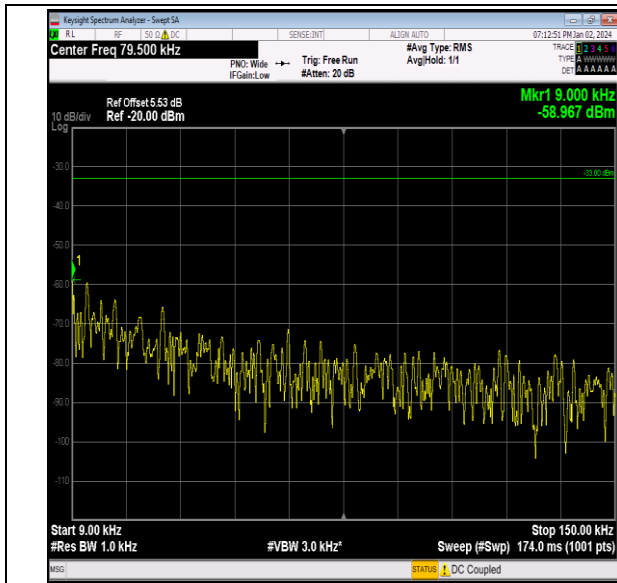
Band13_5MHz_16QAM_23230_1RB#0_0.009~0.15_0.009 ~0.15
