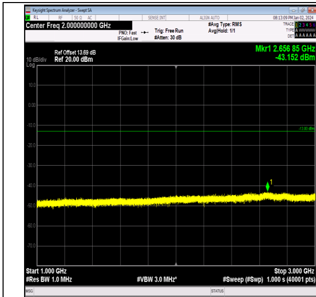
Band26_3MHz_16QAM_26705_1RB#0_1000~3000_1000 ~3000
