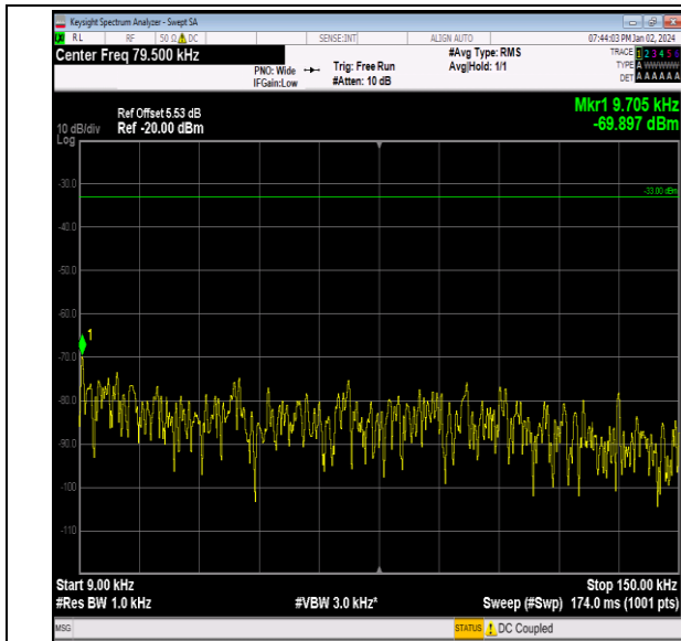
Band26_1.4MHz_QPSK_26697_1RB#0_0.009~0.15_0.00 9~0.15
