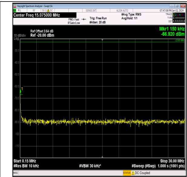
Band26_1.4MHz_16QAM_26740_1RB#0_0.15~30_0.15~ 30
