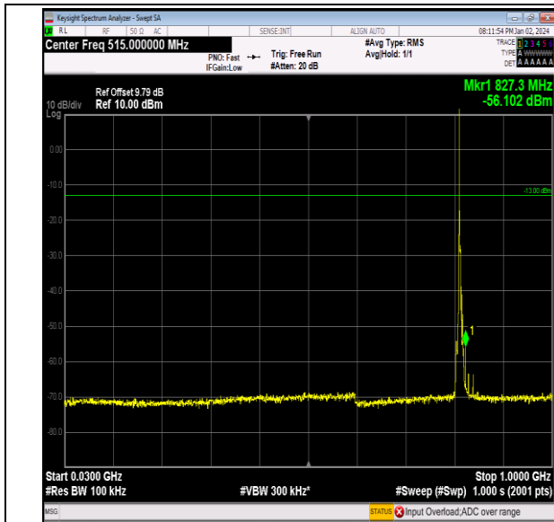
Band26_3MHz_QPSK_26705_1RB#0_30~1000_30~1000
