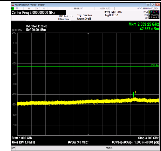
Band26_1.4MHz_16QAM_26740_1RB#0_1000~3000_100 0~3000
