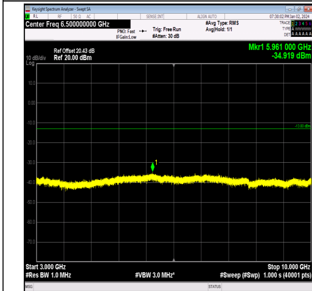
Band13_10MHz_QPSK_23230_1RB#0_3000~10000_300 0~10000
