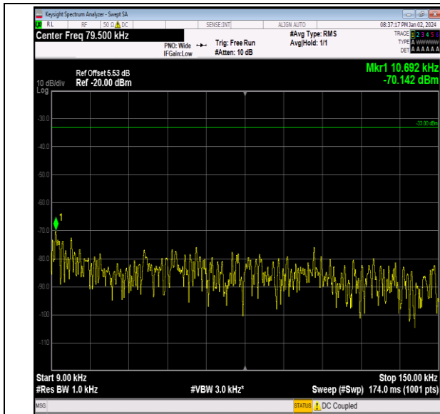
Band26_5MHz_QPSK_26715_1RB#0_0.009~0.15_0.009~0.15
