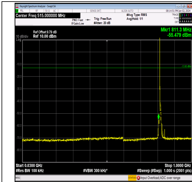
Band26_3MHz_16QAM_26740_1RB#0_30~1000_30~100 0
