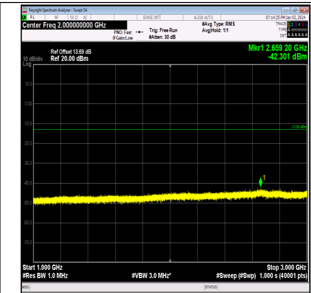
Band13_5MHz_QPSK_23255_1RB#0_1000~3000_1000~3000
