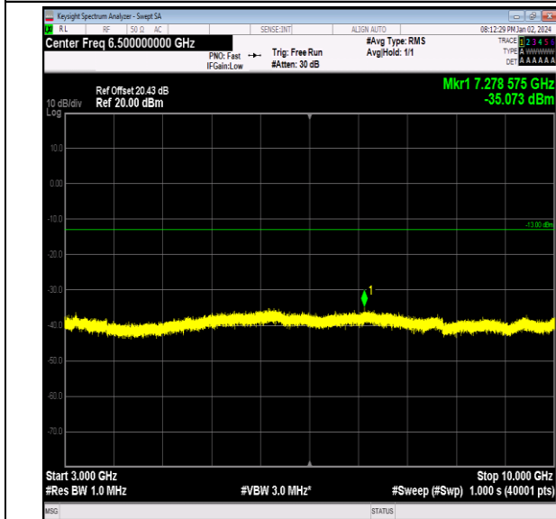
Band26_3MHz_QPSK_26705_1RB#0_3000~10000_3000~10000
