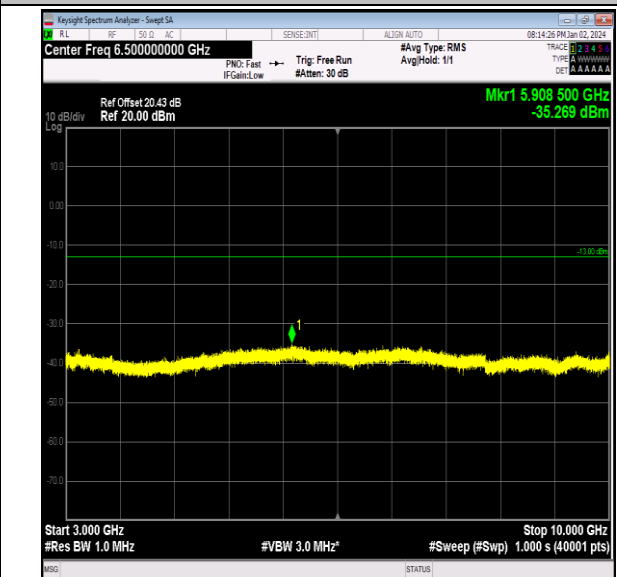
Band26_3MHz_QPSK_26740_1RB#0_3000~10000_3000~10000
