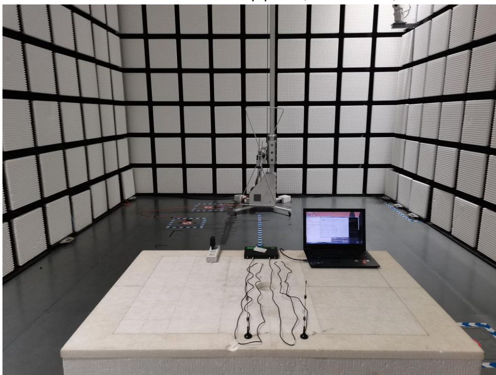
Radiated emission setup photo(30MHz-1GHz)
