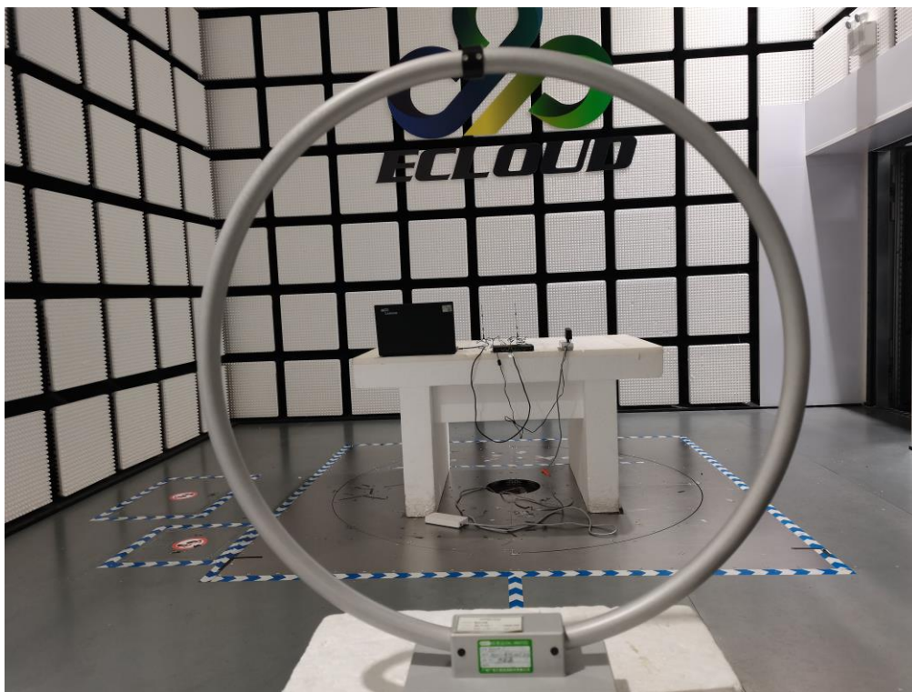
Radiated emission setup photo(Below 30MHz)
