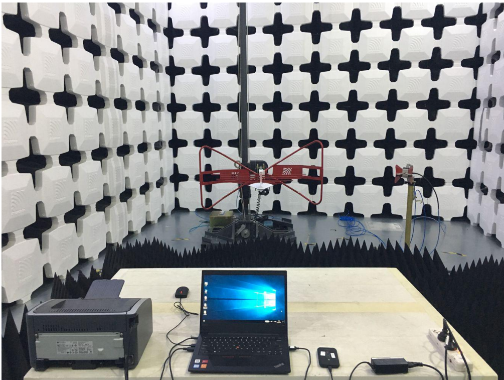
2. Radiated Emissions (Part 15B PC mode)( 1GHz-18GHz)
