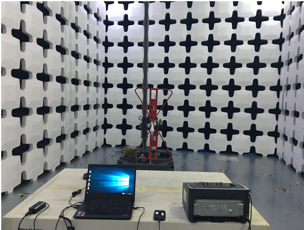
1. Radiated Emissions (Part 15B PC mode) (30MHz- 1GHz)
