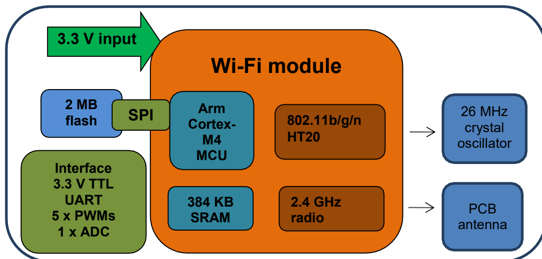
Figure 1-1 WRD8P architecture
