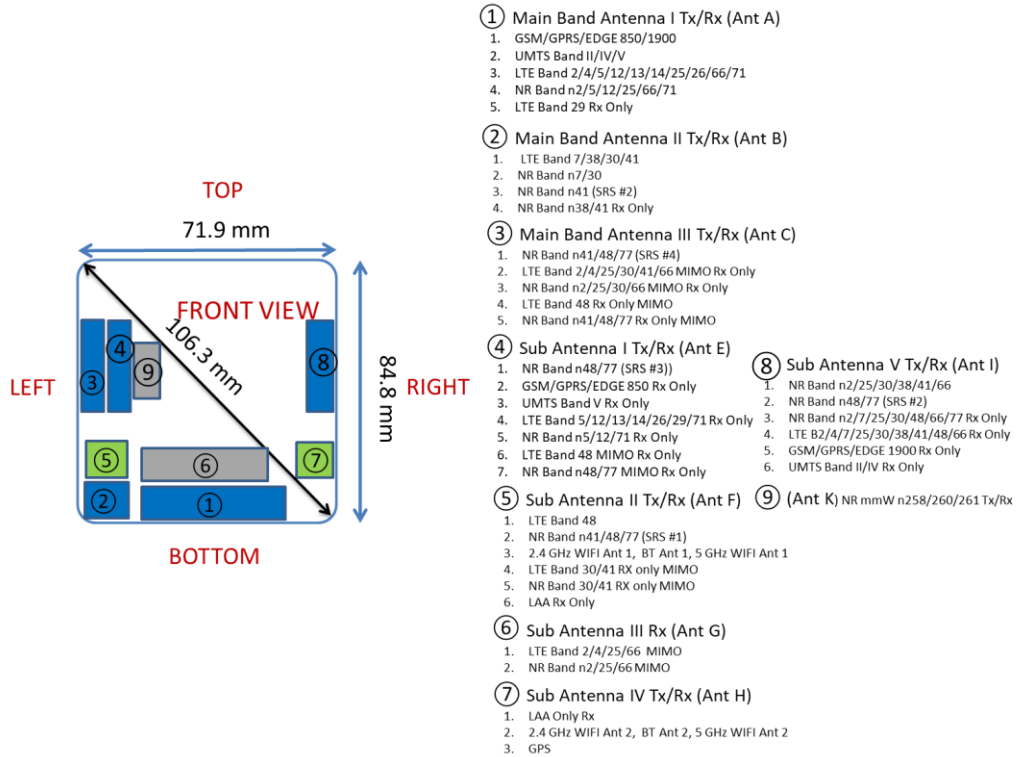
Figure F-1 DUT Antenna Locations Closed Configurations
