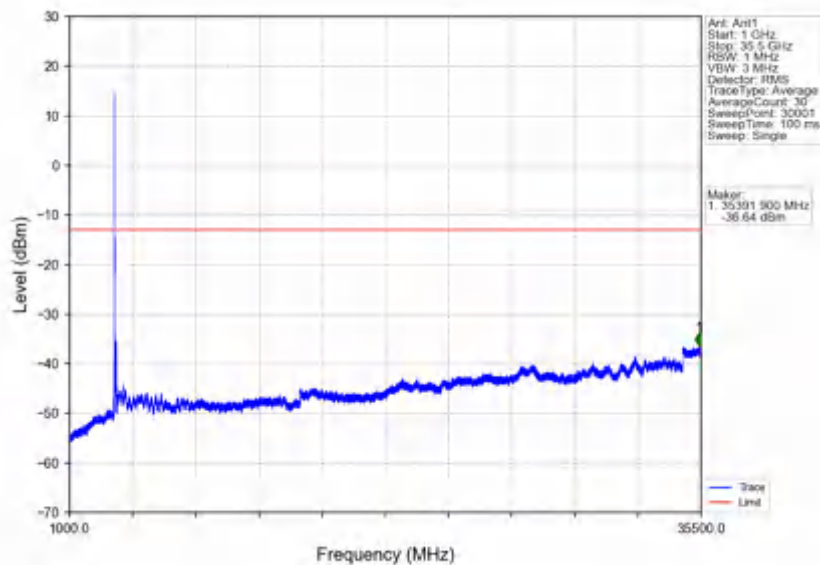
n78e_30kHz_SISO_NTNV_100MHz_DFT-s-OFDM QPSK_3499.98MHz_Edge_1RB_Right
