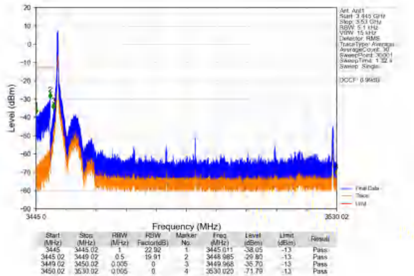
n78e_30kHz_SISO_NTNV_80MHz_DFT-s-OFDM PI/2 BPSK_3490.02MHz_Edge_1RB_Left
