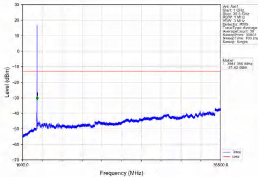
n78e_30kHz_SISO_NTNV_80MHz_CP-OFDM QPSK_3510MHz_Outer_Full
