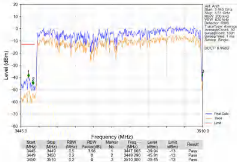
n78e_30kHz_SISO_NTNV_60MHz_DFT-s-OFDM PI/2 BPSK_3480MHz_Outer_Full
