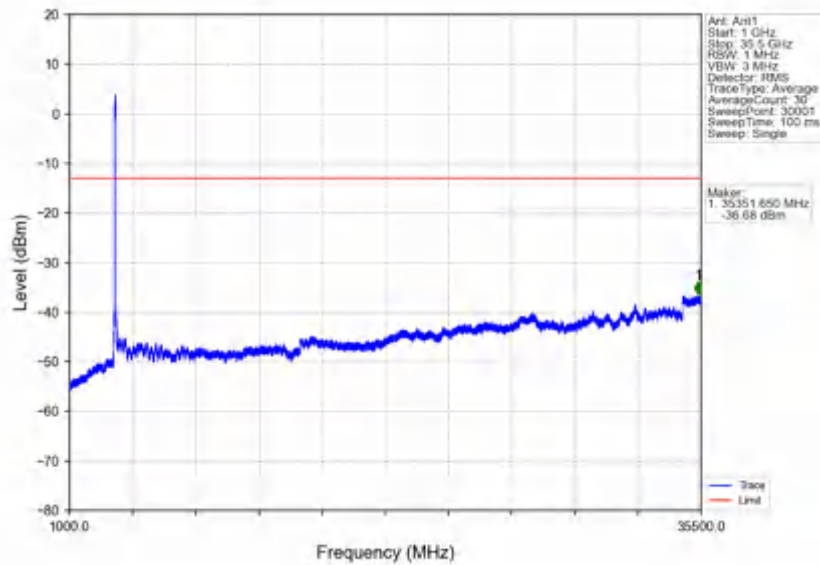
n78e_30kHz_SISO_NTNV_80MHz_DFT-s-OFDM_QPSK_3490.02MHz_Inner_1RB_Left
