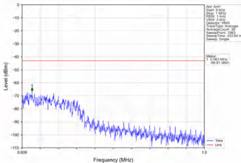
n78e_30kHz_SISO_NTNV_70MHz_CP-OFDM QPSK_3514.98MHz_Edge_1RB_Right
