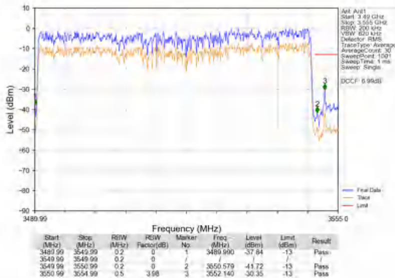
n78e_30kHz_SISO_NTNV_60MHz_CP-OFDM QPSK_3519.99MHz_Outer_Full
