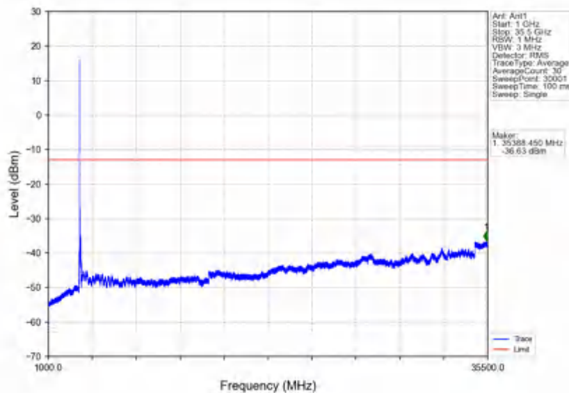
n78e_30kHz_SISO_NTNV_90MHz_CP-OFDM QPSK_3495MHz_Outer_Full
