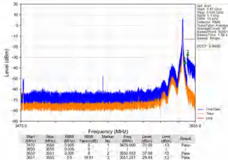
n78e_30kHz_SISO_NTNV_80MHz_CP-OFDM QPSK_3510MHz_Edge_1RB_Right
