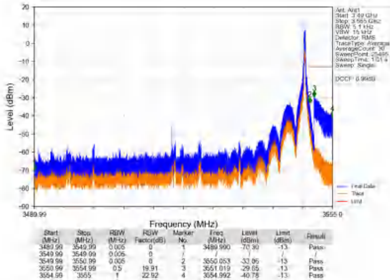
n78e_30kHz_SISO_NTNV_60MHz_DFT-s-OFDM QPSK_3519.99MHz_Edge_1RB_Right
