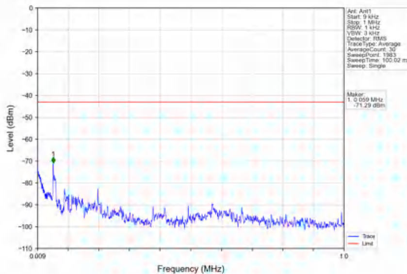
n78e_30kHz_SISO_NTNV_50MHz_DFT-s-OFDM_QPSK_3525MHz_Outer_Full
