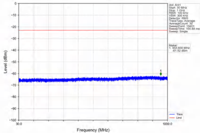
n78e_30kHz_SISO_NTNV_70MHz_CP-OFDM QPSK_3485.01MHz_Outer_Full
