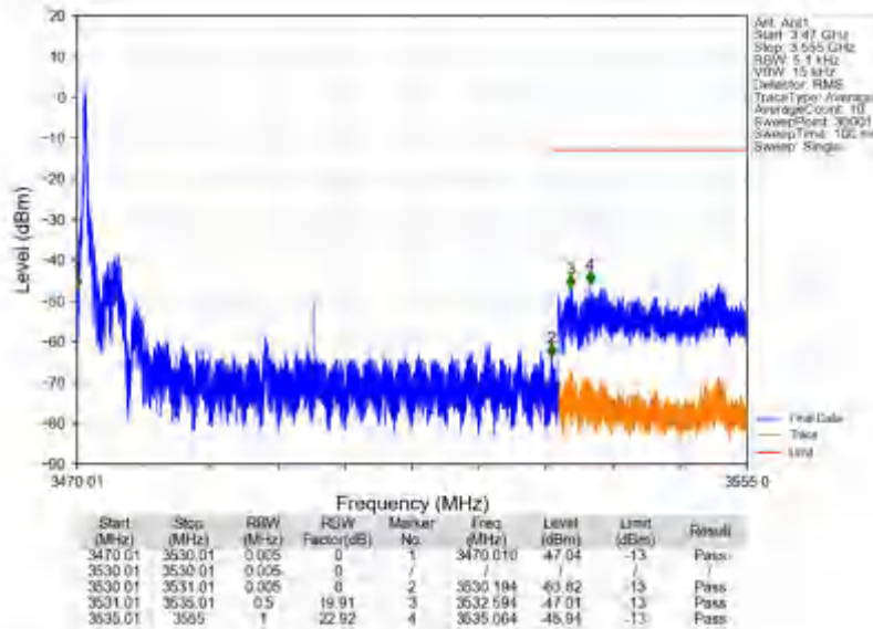
n78e_30kHz_SISO_NTV_60MHz_CP-OFDM QPSK_3500.01MHz_Edge_1RB_Left
