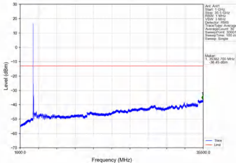
n78e_30kHz_SISO_NTV_90MHz_DFT-s-OFDM QPSK_3495MHz_Edge_1RB_Left
