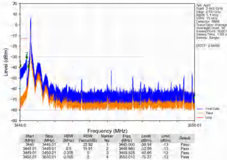
n78e_30kHz_SISO_NTNV_100MHz_DFT-s-OFDM QPSK_3500.01MHz_Inner_1RB_Left
