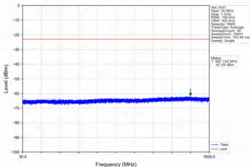
n78e_30kHz_SISO_NTNV_90MHz_DFT-s-OFDM QPSK_3504.99MHz_Inner_1RB_Right
