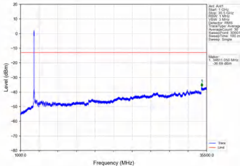
n78e_30kHz_SISO_NTNV_90MHz_CP-OFDM_QPSK_3495MHz_Outer_Full
