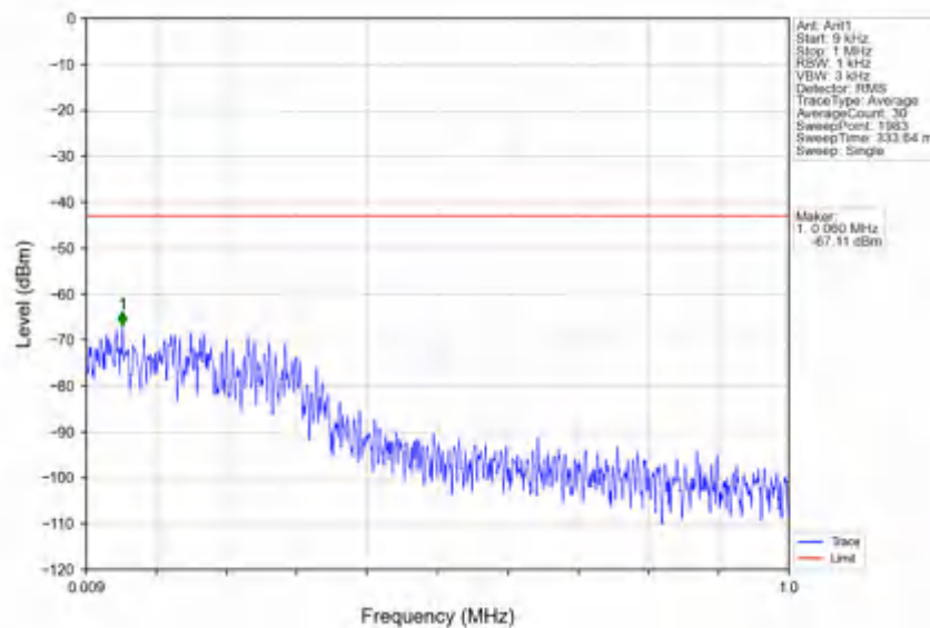
n78e_30kHz_SISO_NTNV_80MHz_CP-OFDM QPSK_3510MHz_Edge_1RB_Right
