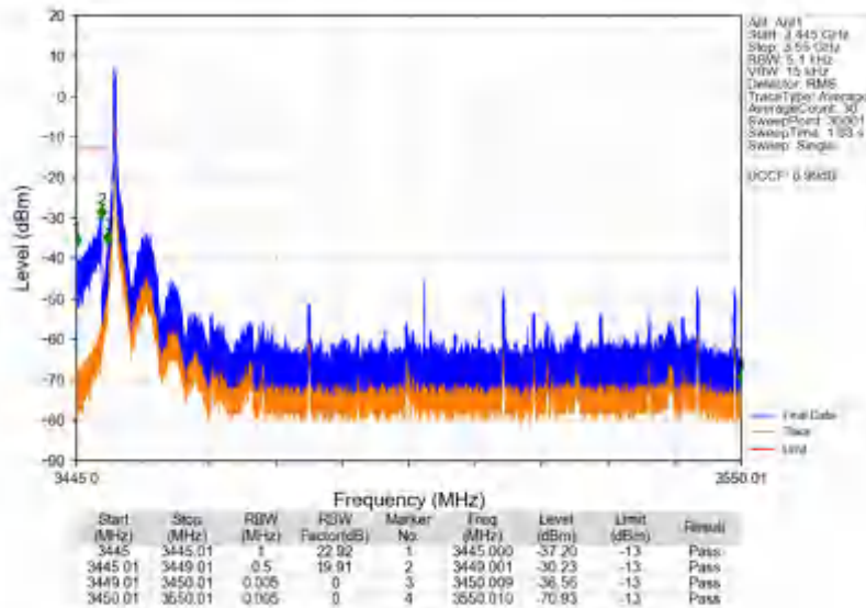
n78e_30kHz_SISO_NTNV_100MHz_DFT-s-OFDM QPSK_3500.01MHz_Edge_1RB_Left
