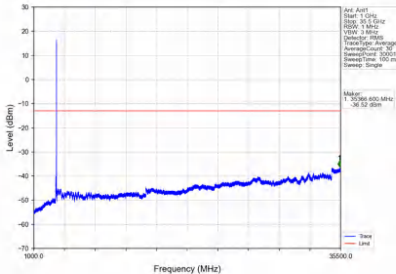
n78e_30kHz_SISO_NTNV_80MHz_DFT-s-OFDM QPSK_3510MHz_Edge_1RB_Right
