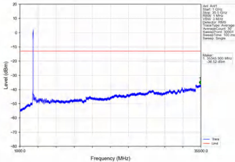
n78e_30kHz_SISO_NTNV_100MHz_DFT-s-OFDM QPSK_3500.01MHz_Inner_1RB_Left
