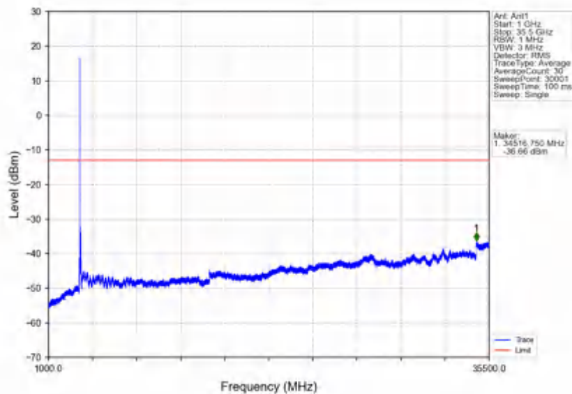
n78e_30kHz_SISO_NTV_80MHz_CP-OFDM QPSK_3490.02MHz_Outer_Full
