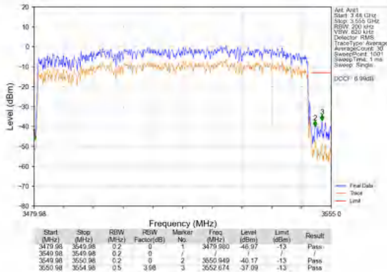
n78e_30kHz_SISO_NTNV_70MHz_CP-OFDM QPSK_3514.98MHz_Outer_Full
