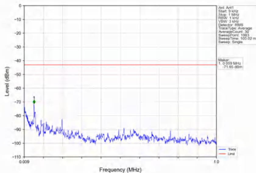
n78e_30kHz_SISO_NTNV_90MHz_DFT-s-OFDM_QPSK_3495MHz_Outer_Full
