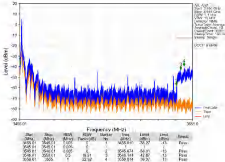
n78e_30kHz_SISO_NTNV_90MHz_DFT-s-OFDM PI/2 BPSK_3500.01MHz_Edge_1RB_Left
