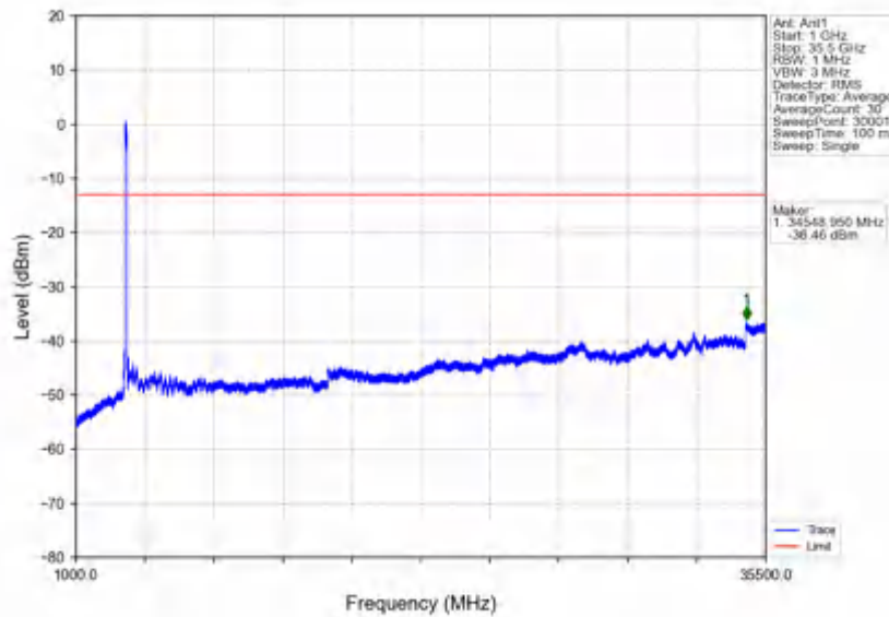
n78e_30kHz_SISO_NTNV_100MHz_DFT-s-OFDM QPSK_3499.98MHz_Inner_1RB_Right
