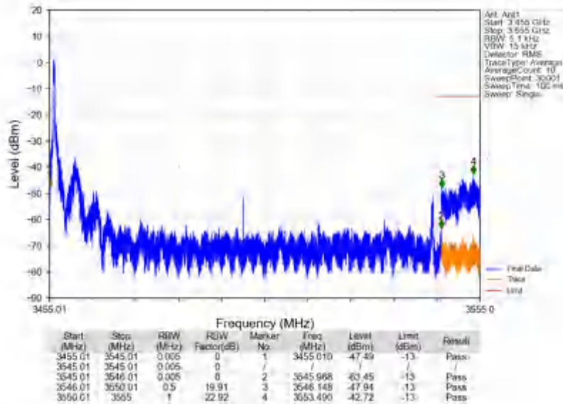
n78e_30kHz_SISO_NTV_90MHz_CP-OFDM QPSK_3500.01MHz_Edge_1RB_Left
