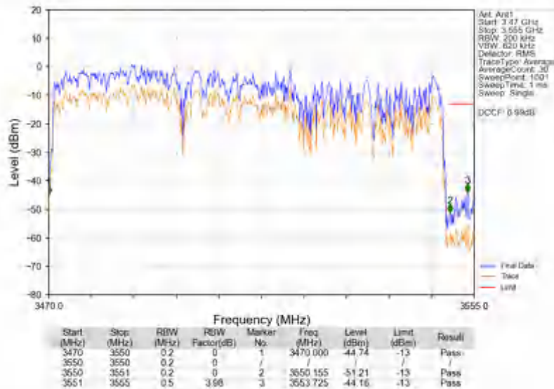
n78e_30kHz_SISO_NTNV_80MHz_DFT-s-OFDM PI/2 BPSK_3510MHz_Outer_Full
