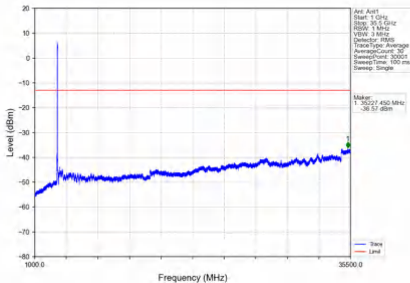
n78e_30kHz_SISO_NTNV_50MHz_DFT-s-OFDM_QPSK_3475.02MHz_Inner_1RB_Left
