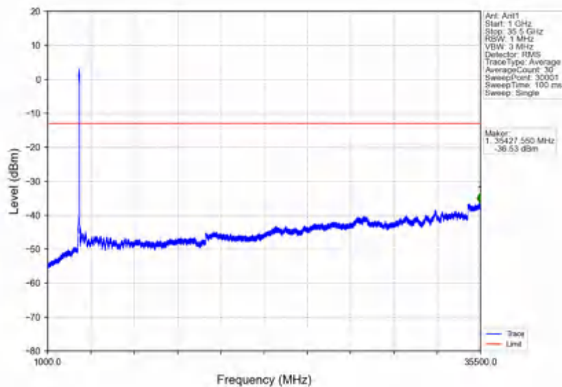
n78e_30kHz_SISO_NTNV_80MHz_DFT-s-OFDM QPSK_3510MHz_Inner_1RB_Right
