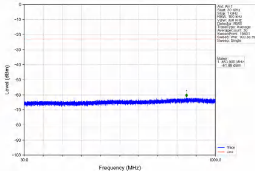
n78e_30kHz_SISO_NTNV_60MHz_DFT-s-OFDM_QPSK_3480MHz_Outer_Full
