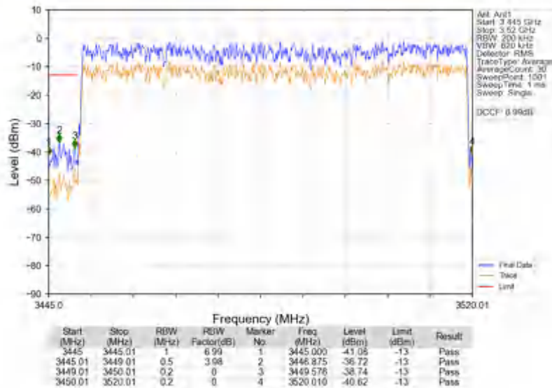
n78e_30kHz_SISO_NTNV_70MHz_CP-OFDM_QPSK_3485.01MHz_Outer_Full
