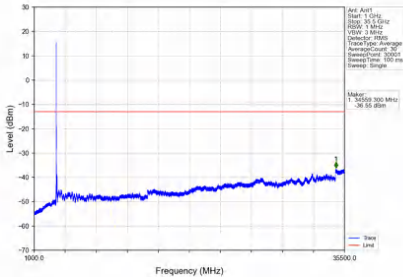
n78e_30kHz_SISO_NTNV_90MHz_DFT-s-OFDM PI/2 BPSK_3495MHz_Outer_Full
