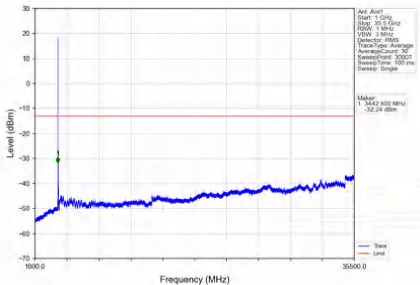
n78e_30kHz_SISO_NTNV_60MHz_DFT-s-OFDM PI/2 BPSK_3480MHz_Outer_Full
