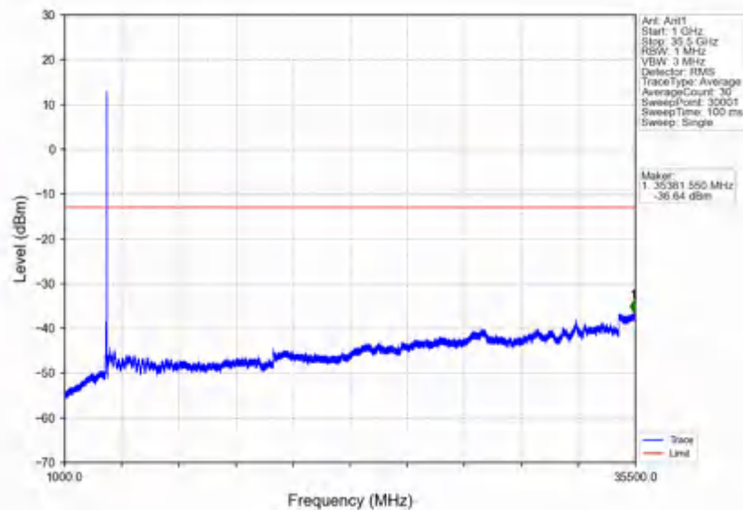
n78e_30kHz_SISO_NTNV_50MHz_CP-OFDM QPSK_3525MHz_Outer_Full
