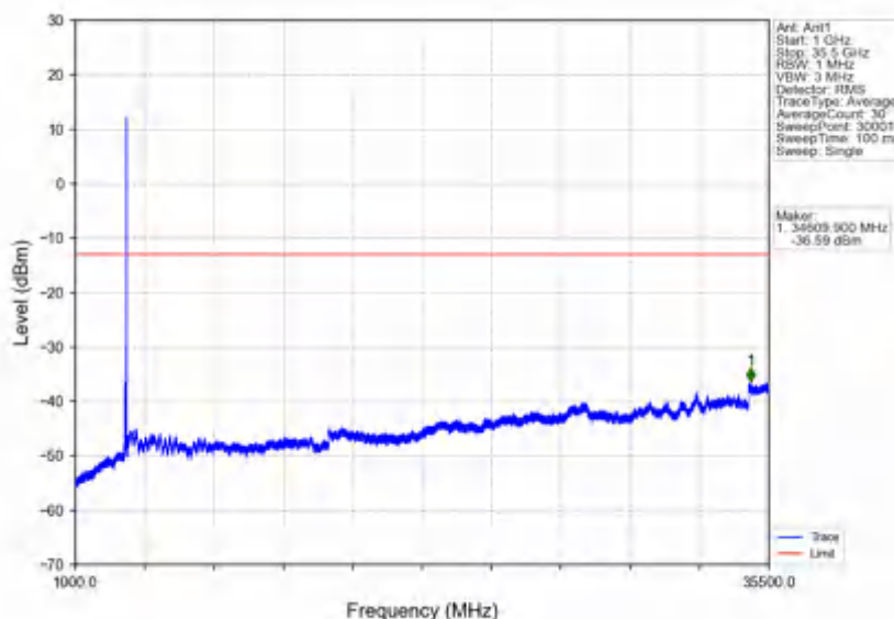
n78e_30kHz_SISO_NTNV_90MHz_DFT-s-OFDM QPSK_3504.99MHz_Edge_1RB_Right
