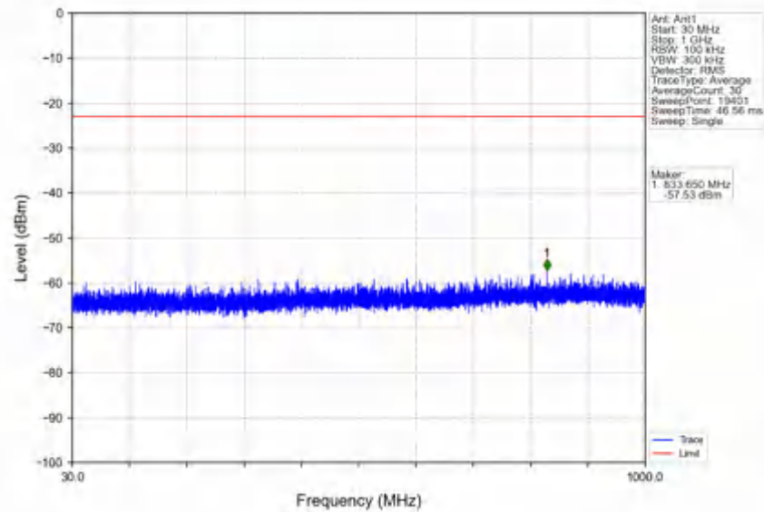
n78e_30kHz_SISO_NTV_60MHz_DFT-s-OFDM_QPSK_3480MHz_Edge_1RB_Left
