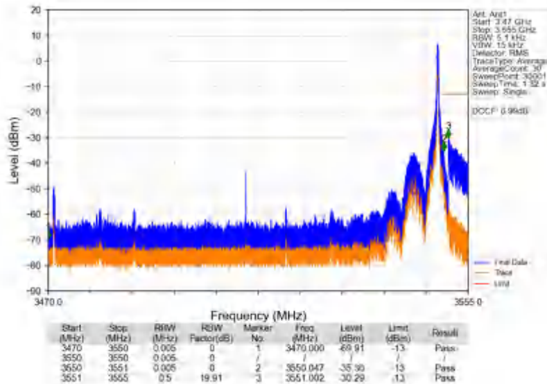
n78e_30kHz_SISO_NTNV_80MHz_DFT-s-OFDM QPSK_3510MHz_Edge_1RB_Right
