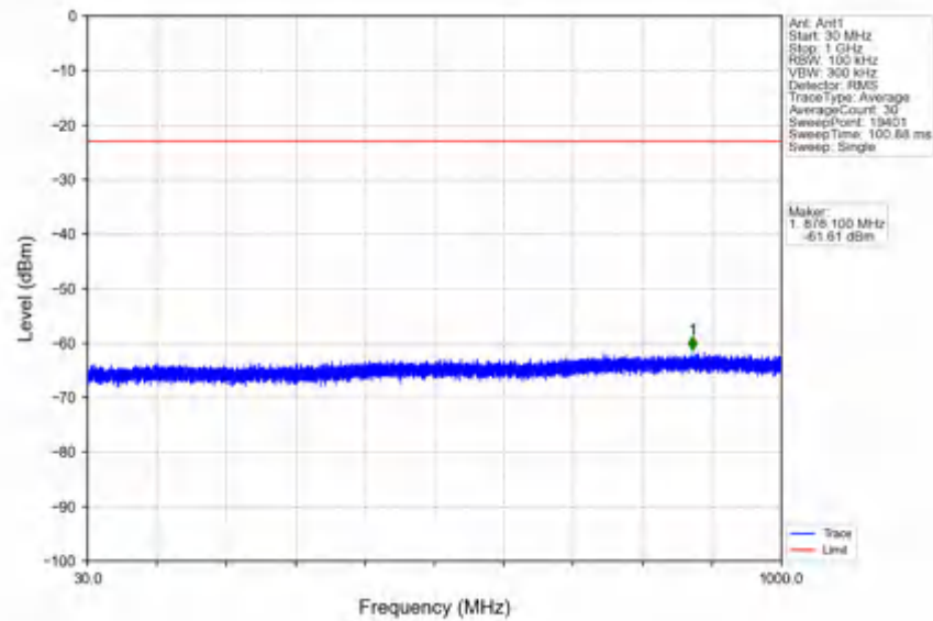
n78e_30kHz_SISO_NTNV_90MHz_CP-OFDM QPSK_3504.99MHz_Outer_Full
