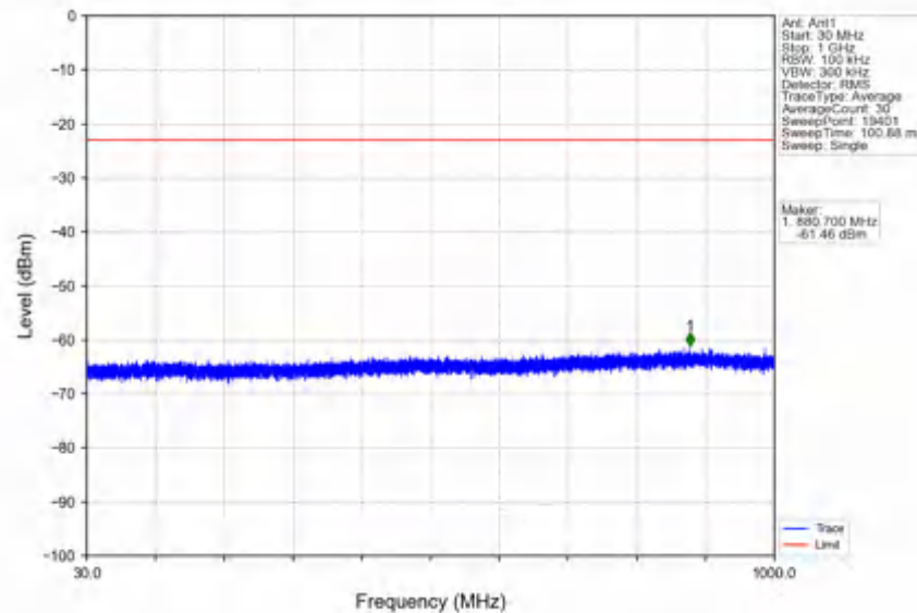
n78e_30kHz_SISO_NTNV_70MHz_CP-OFDM QPSK_3514.98MHz_Inner_1RB_Right
