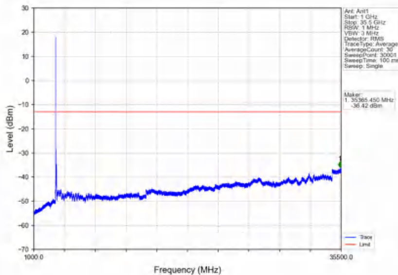
n78e_30kHz_SISO_NTV_90MHz_CP-OFDM QPSK_3500.01MHz_Edge_1RB_Left
