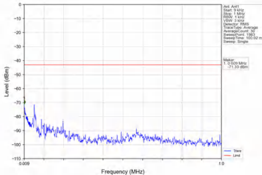
n78e_30kHz_SISO_NTNV_80MHz_DFT-s-OFDM_QPSK_3490.02MHz_Outer_Full
