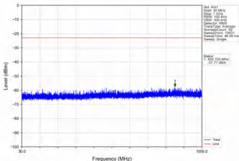
n78e_30kHz_SISO_NTNV_80MHz_CP-OFDM QPSK_3510MHz_Edge_1RB_Right
