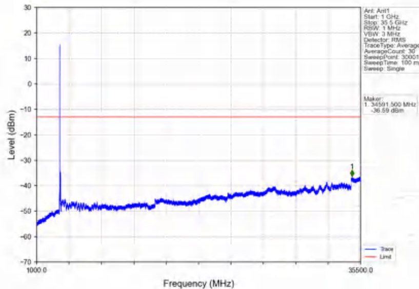
n78e_30kHz_SISO_NTNV_90MHz_DFT-s-OFDM PI/2 BPSK_3500.01MHz_Edge_1RB_Left
