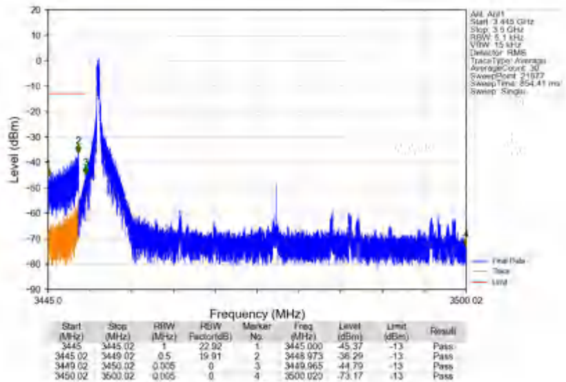
n78e_30kHz_SISO_NTNV_50MHz_DFT-s-OFDM_QPSK_3475.02MHz_Inner_1RB_Left
