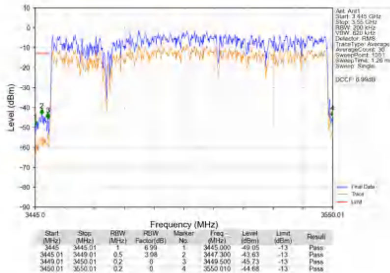
n78e_30kHz_SISO_NTNV_100MHz_DFT-s-OFDM_PI/2_BPSK_3500.01MHz_Outer_Full
