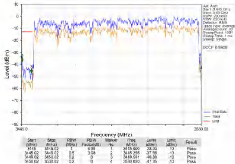
n78e_30kHz_SISO_NTNV_80MHz_DFT-s-OFDM_QPSK_3490.02MHz_Outer_Full
