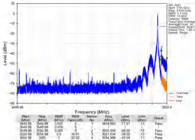
n78e_30kHz_SISO_NTNV_100MHz_DFT-s-OFDM QPSK_3499.98MHz_Inner_1RB_Right
