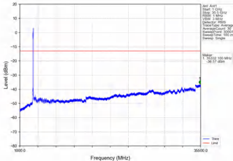
n78e_30kHz_SISO_NTNV_80MHz_CP-OFDM_QPSK_3510MHz_Outer_Full
