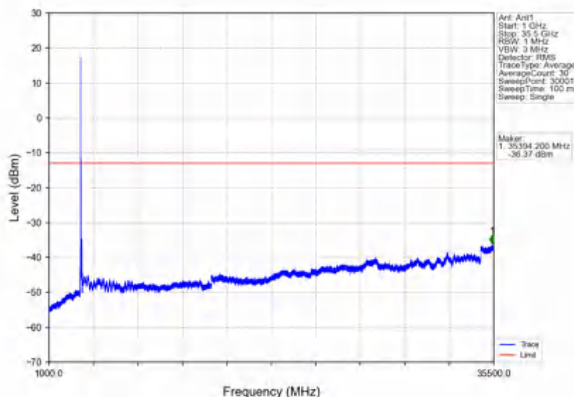
n78e_30kHz_SISO_NTNV_100MHz_DFT-s-OFDM QPSK_3500.01MHz_Edge_1RB_Left
