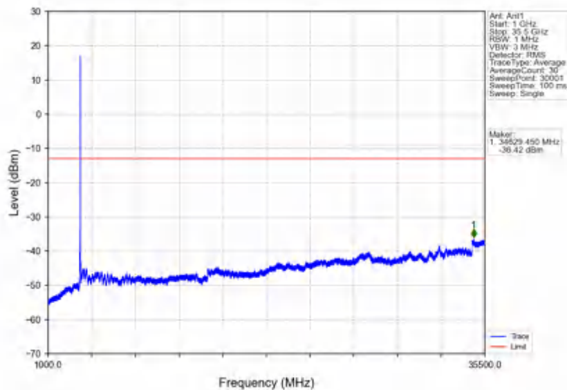
n78e_30kHz_SISO_NTNV_60MHz_CP-OFDM QPSK_3519.99MHz_Outer_Full
