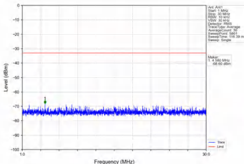
n78e_30kHz_SISO_NTNV_70MHz_DFT-s-OFDM QPSK_3514.98MHz_Edge_1RB_Right
