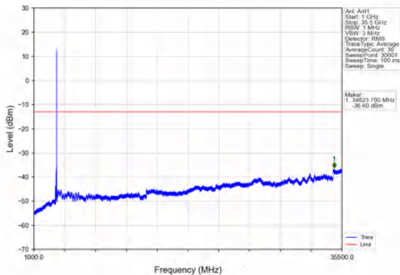
n78e_30kHz_SISO_NTNV_80MHz_DFT-s-OFDM PI/2 BPSK_3510MHz_Outer_Full
