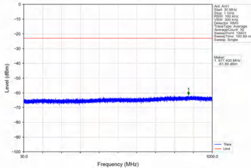
n78e_30kHz_SISO_NTNV_90MHz_DFT-s-OFDM PI/2 BPSK_3495MHz_Outer_Full
