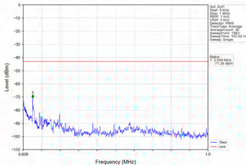
n78e_30kHz_SISO_NTNV_70MHz_DFT-s-OFDM_QPSK_3514.98MHz_Outer_Full
