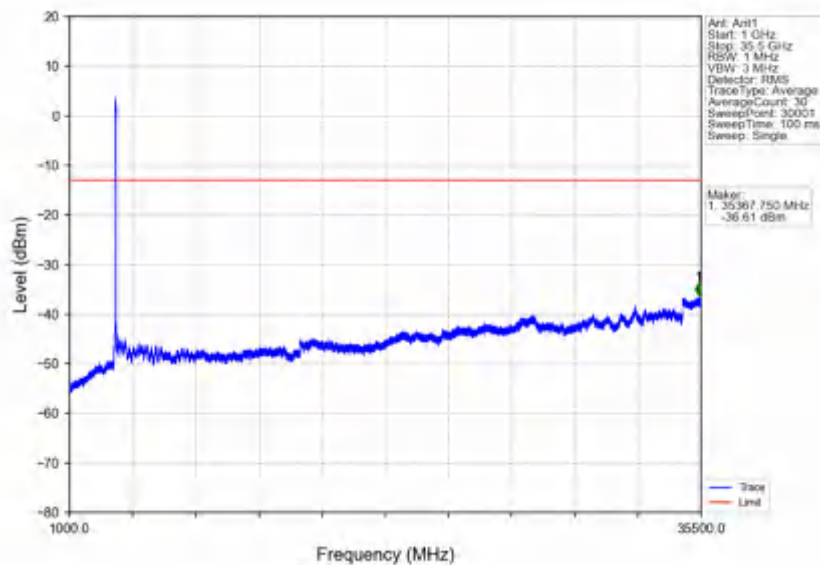
n78e_30kHz_SISO_NTNV_70MHz_DFT-s-OFDM_QPSK_3514.98MHz_Inner_1RB_Right
