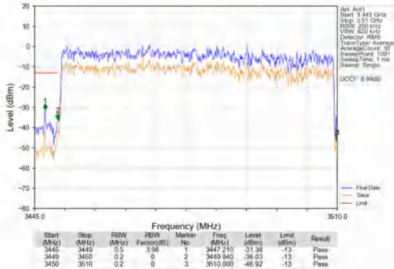
n78e_30kHz_SISO_NTNV_60MHz_CP-OFDM QPSK_3480MHz_Outer_Full
