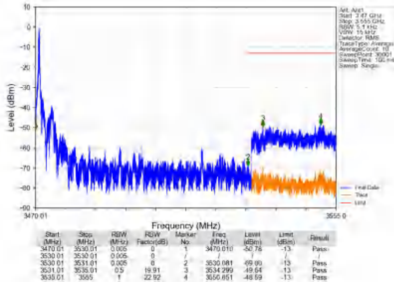
n78e_30kHz_SISO_NTNV_60MHz_DFT-s-OFDM PI/2 BPSK_3500.01MHz_Edge_1RB_Left
