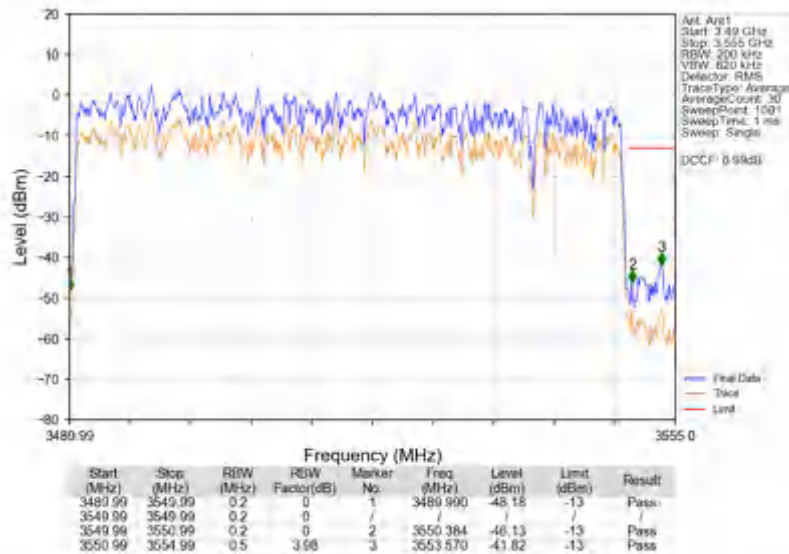
n78e_30kHz_SISO_NTNV_60MHz_DFT-s-OFDM_QPSK_3519.99MHz_Outer_Full
