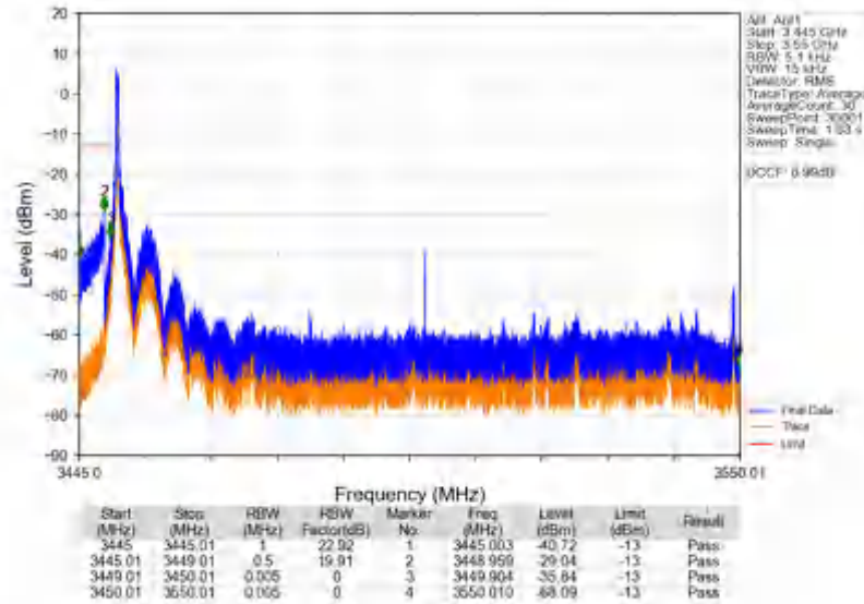
n78e_30kHz_SISO_NTNV_100MHz_CP-OFDM QPSK_3500.01MHz_Edge_1RB_Left
