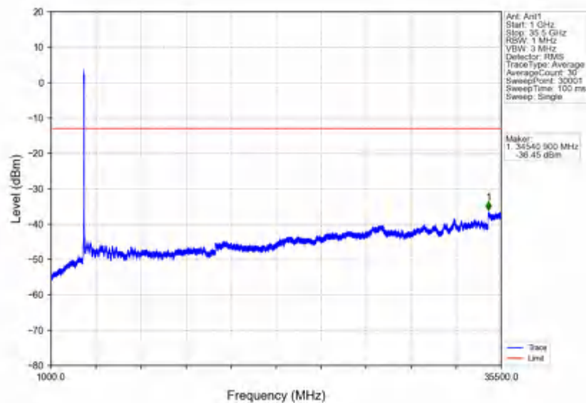
n78e_30kHz_SISO_NTNV_50MHz_DFT-s-OFDM QPSK_3525MHz_Inner_1RB_Right
