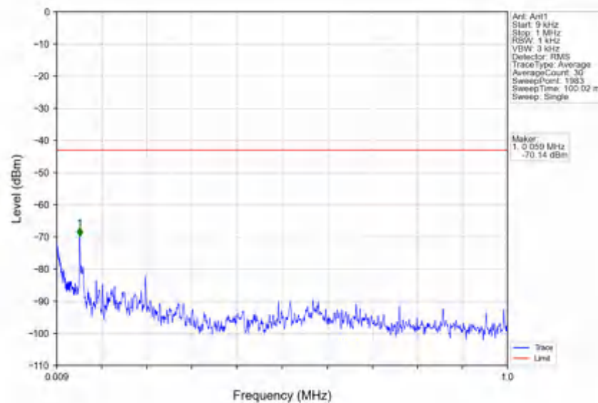
n78e_30kHz_SISO_NTNV_80MHz_DFT-s-OFDM_QPSK_3510MHz_Outer_Full
