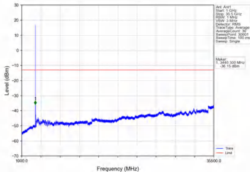
n78e_30kHz_SISO_NTNV_60MHz_DFT-s-OFDM PI/2 BPSK_3500.01MHz_Edge_1RB_Left
