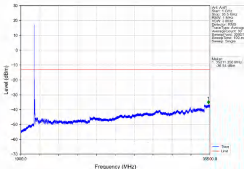
n78e_30kHz_SISO_NTNV_100MHz_CP-OFDM QPSK_3500.01MHz_Edge_1RB_Left
