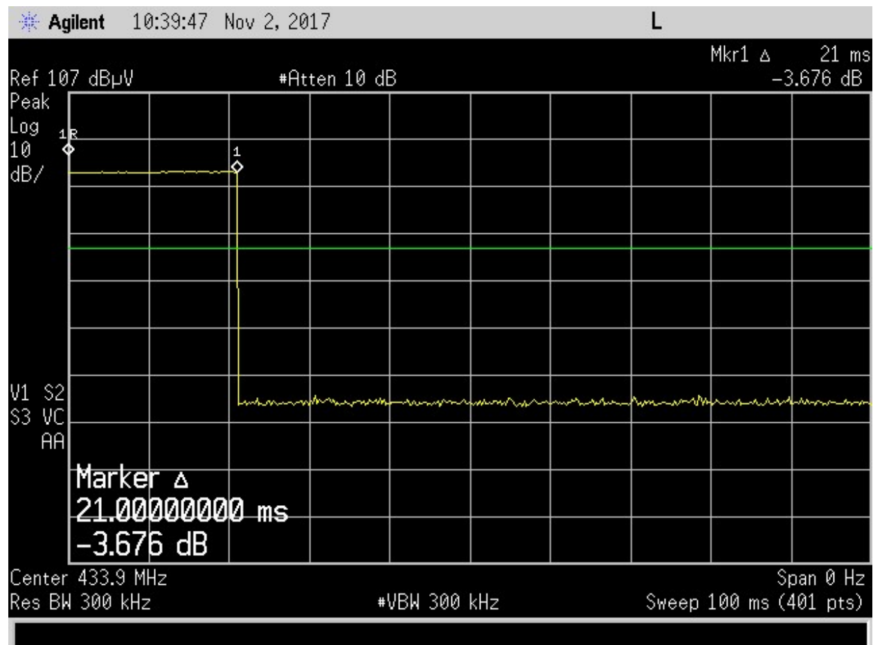
Figure 3. Duty Cycle
