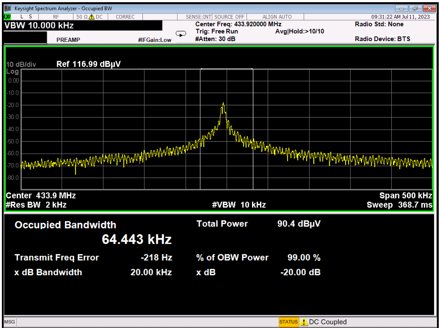
99% Bandwidth Plot – With External Sensor Adapter
