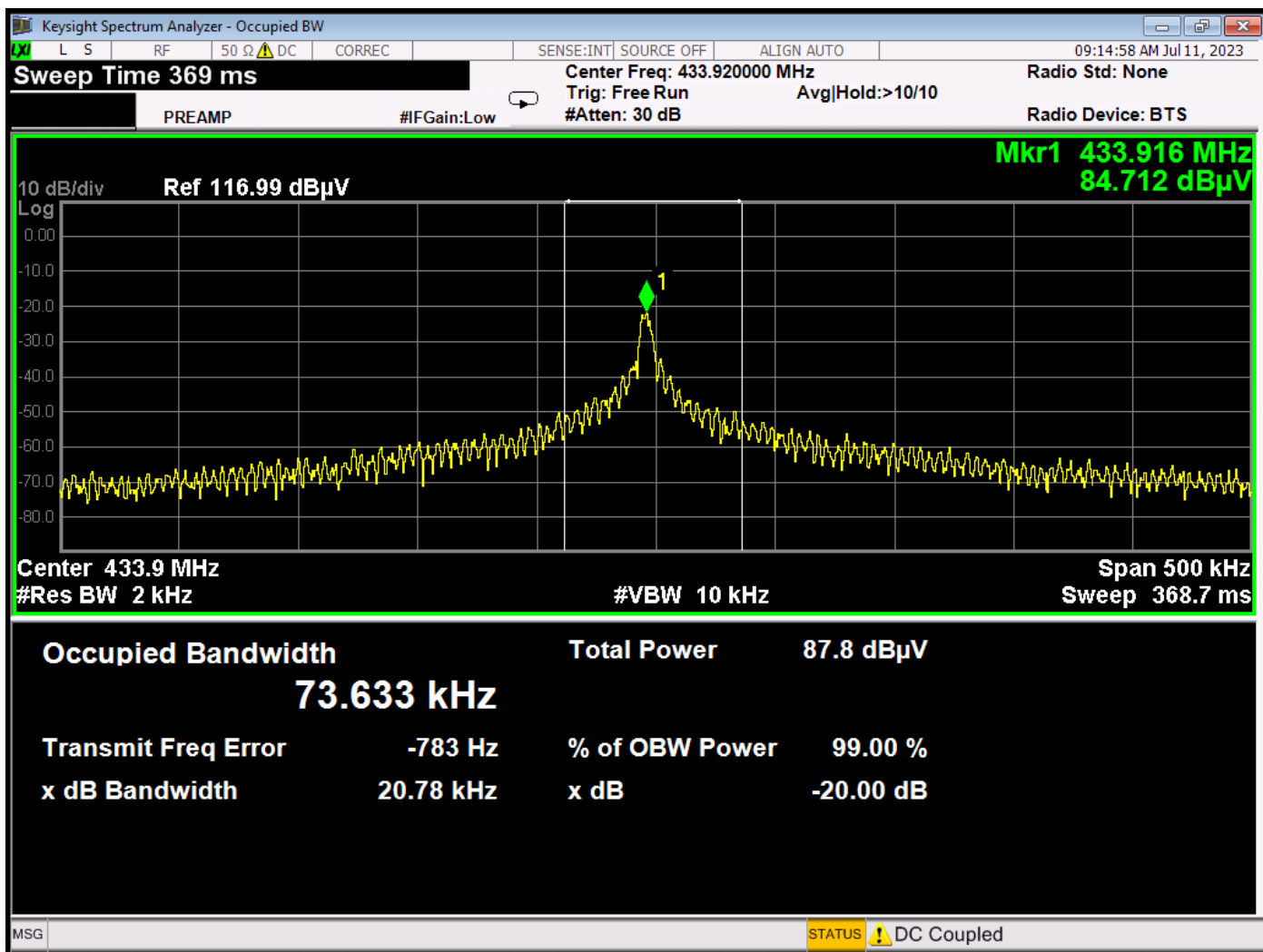
99% Bandwidth Plot – No External Sensor Adapter
