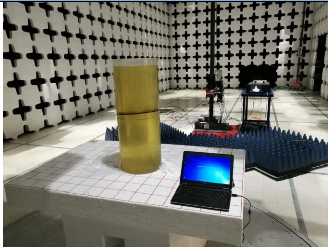
Radiated Emissions (1GHz-6GHz) – Front View
