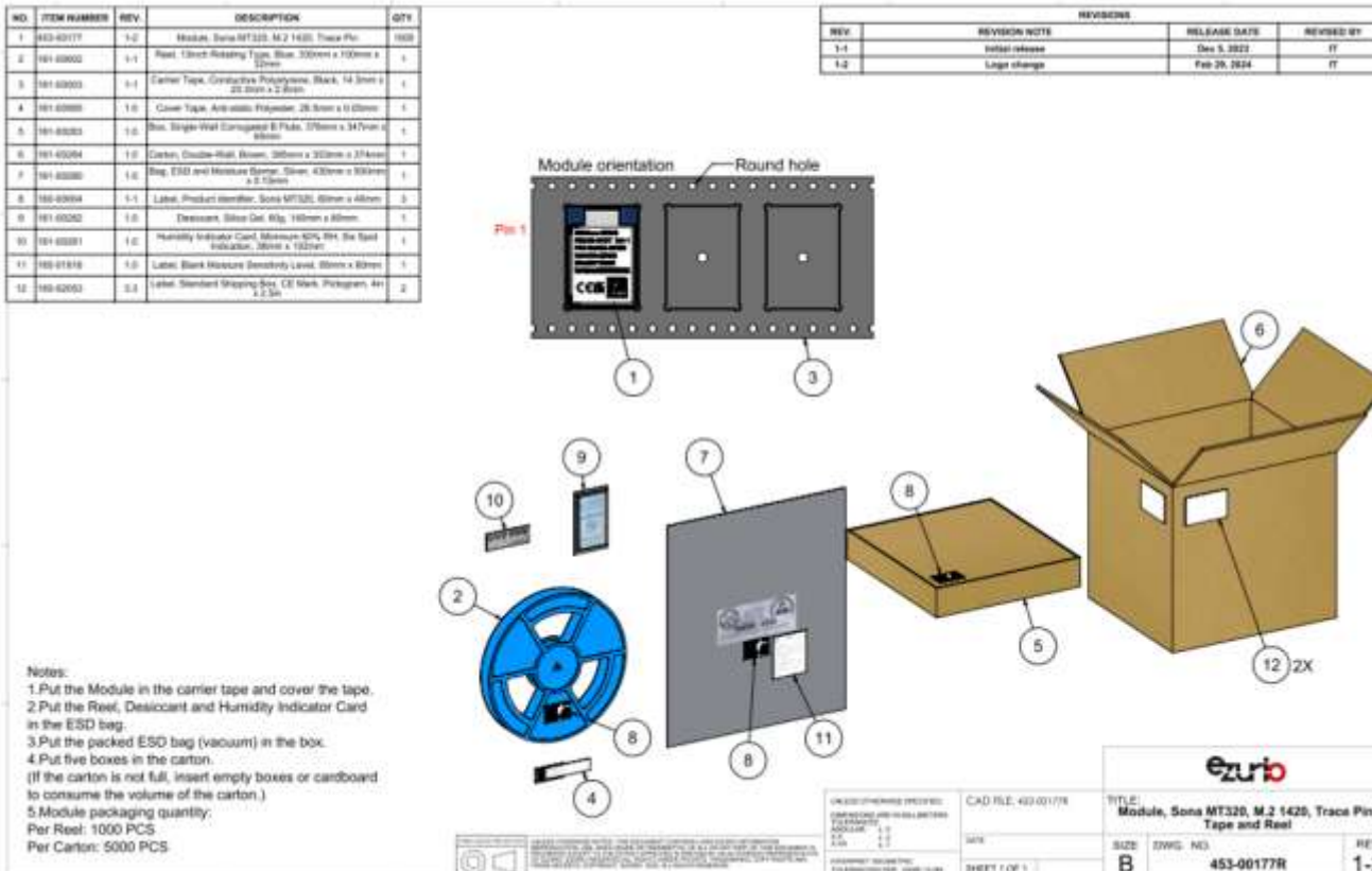
Figure 8: Sona MT320 M.2 1420 packaging processes
