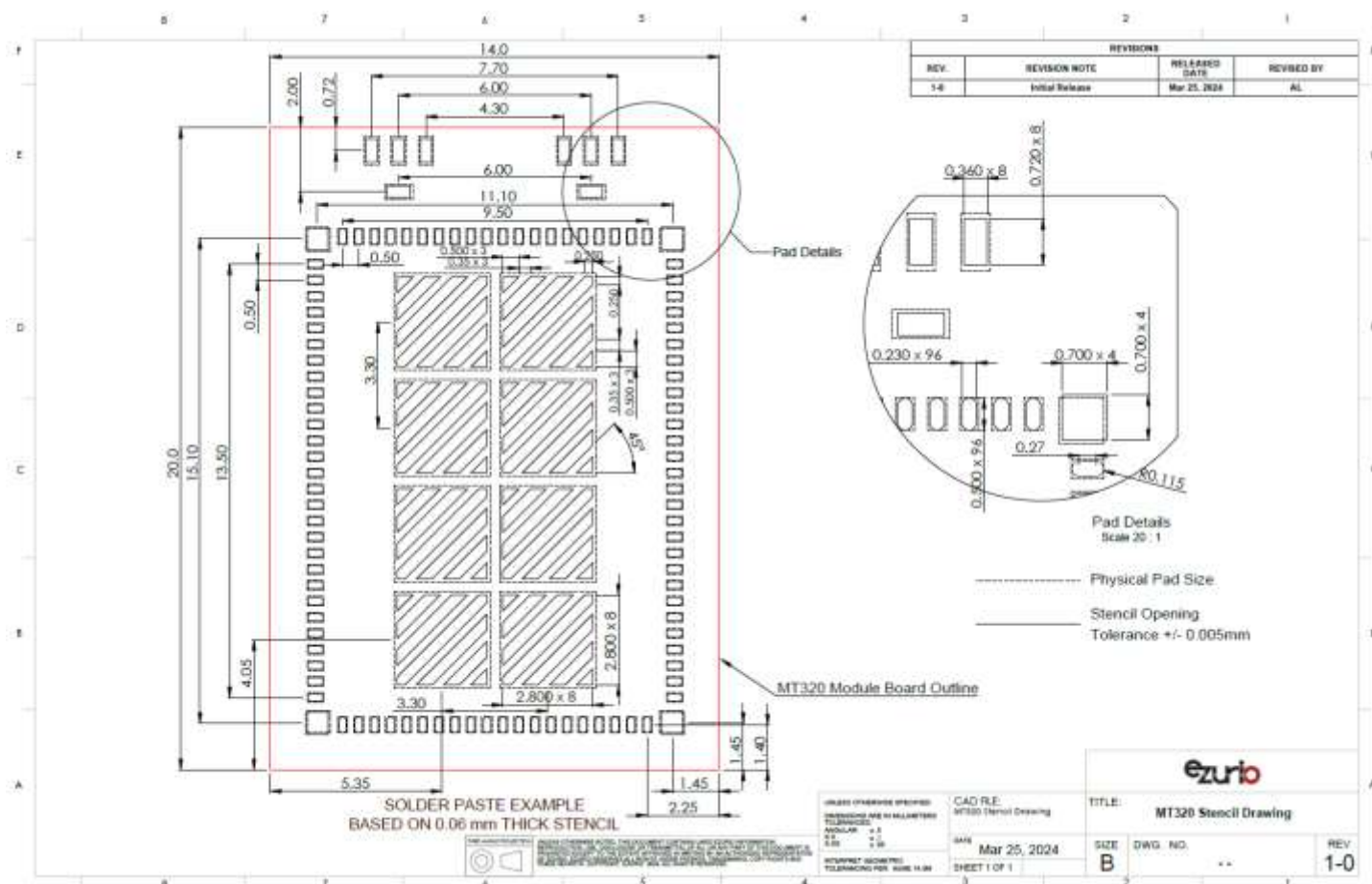
Figure 22: Sona MT320 M.2 1420 recommend stencil design
