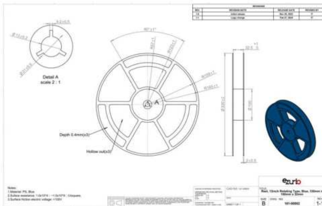
Figure 6: Sona MT320 M.2 1420 Reel specifications, 161-00002
