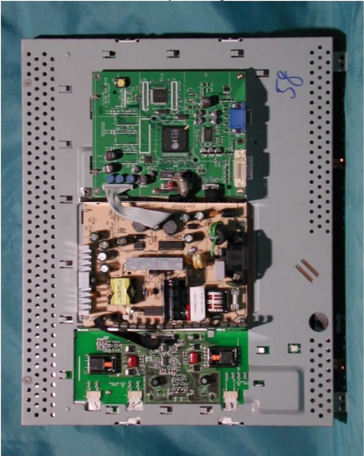
Panel Assembly w/o Shielding Cover
