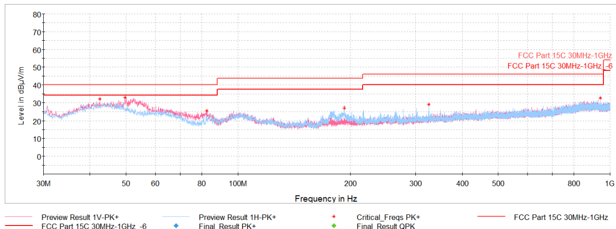
Plot 7-97. Radiated Spurious Emissions Below 1GHz TxBF (1Mbps, ePA – Ch.19, Pol. H & V, with AC/DC Adapter)
