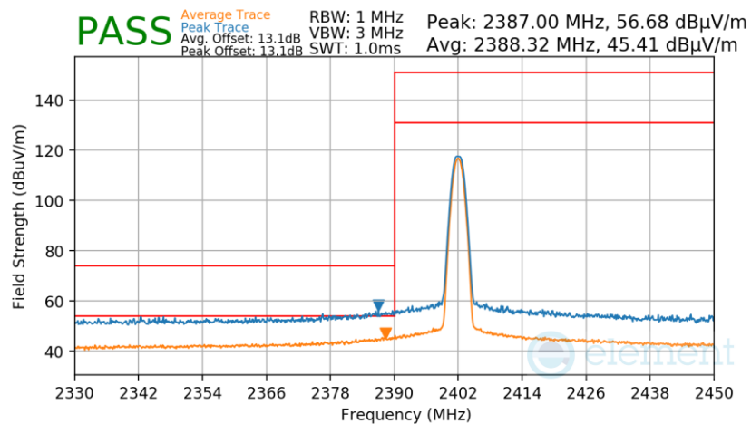
Plot 7-85. Radiated Restricted Lower Band Edge Measurement Antenna WF8 (Average & Peak)
