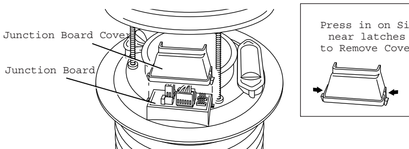
Junction Board Cover Installation
