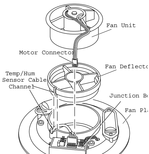
Sensor Cable Channel in Fan Plate and Fan Deflector
