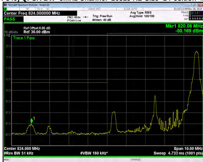
Band26(824-849) QPSK BW=5MHz Channel=26815 RB Size=1 Position=#0 Extended
