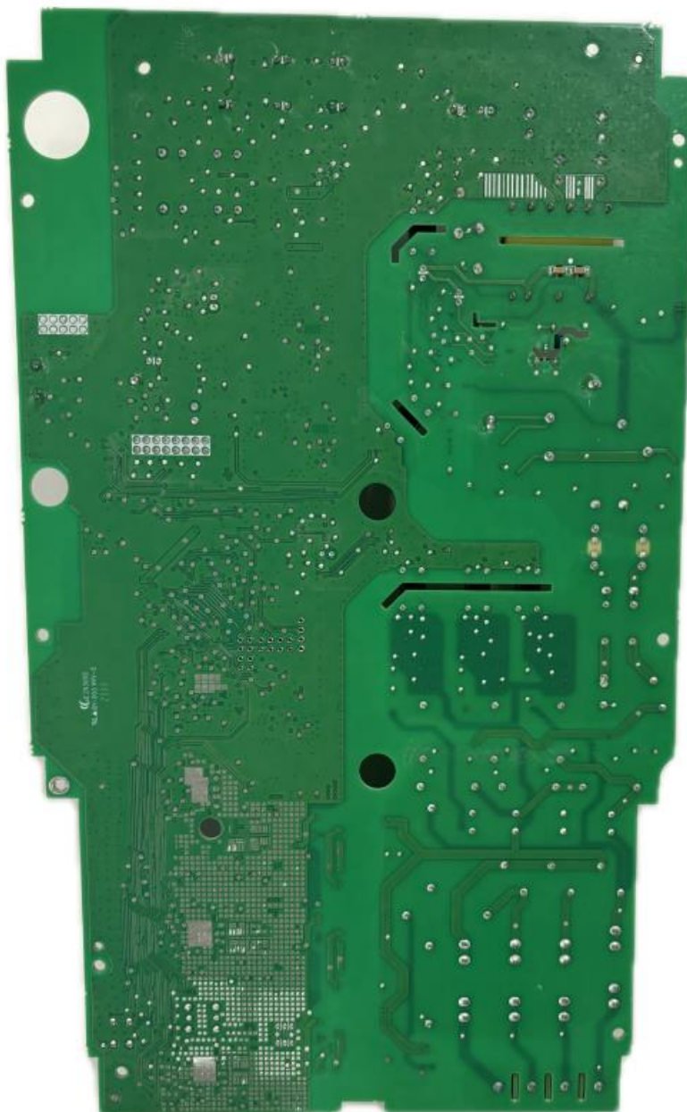
Figure 3 - LVM G3 Hybrid GL0 extension board HW version KF21J027 V4.0 bottom
