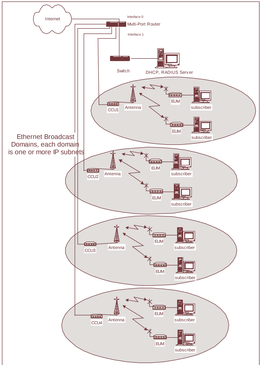
Figure 35 Switched Ethernet Mode – using multi-port router
