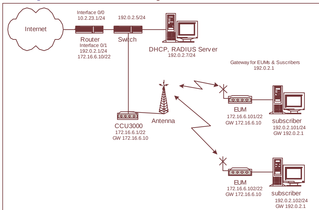
Figure 14 Switched Ethernet Mode with Multiple Subnets
