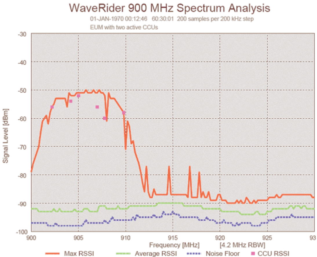
Figure 1 Sample WaveRider 900 MHz Spectral Analysis
