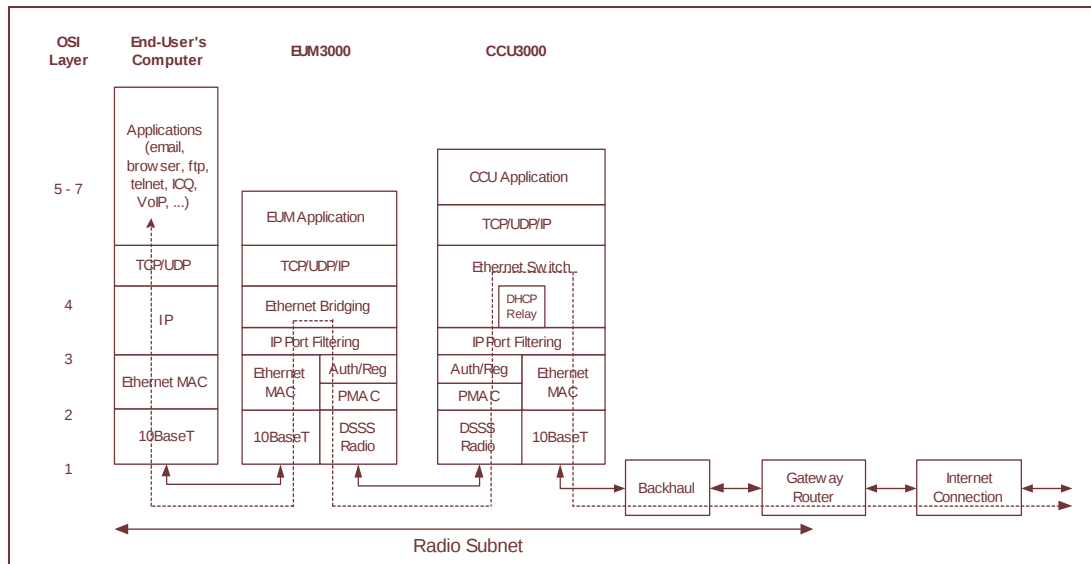
Figure 19 Switched Ethernet Mode and Through Only Mode
