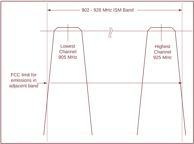
Figure 22 Determination of Lowest and Highest Channel
