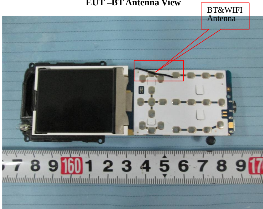
EUT –BT Antenna View
