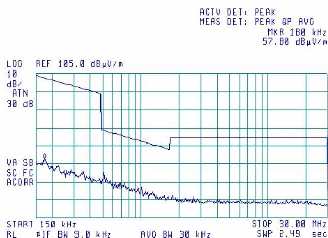
Plot 7.5.12 Radiated emission measurements from 0.15 to 30 MHz at the 5.805GHz carrier frequency
