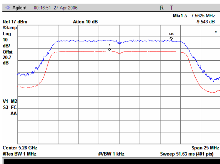
Plot 7.4.2 Peak excursion measurements at 5.260 GHz, 6 Mbps
