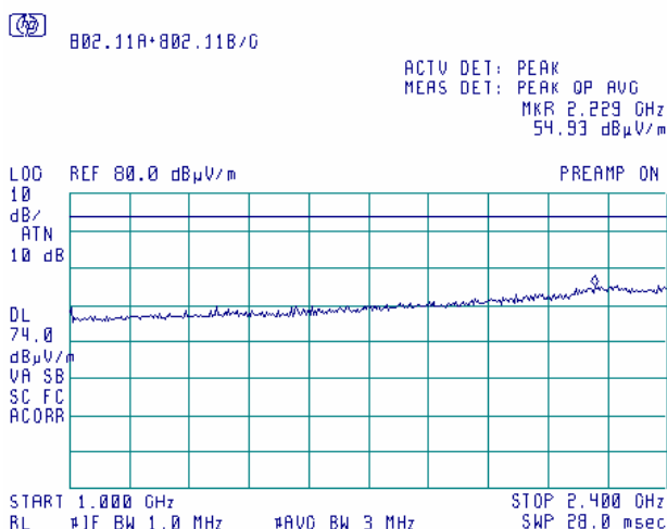
Plot 7.5.77 Radiated emission measurements from 1.0 to 2.4 GHz at the 5.745 GHz carrier frequency
