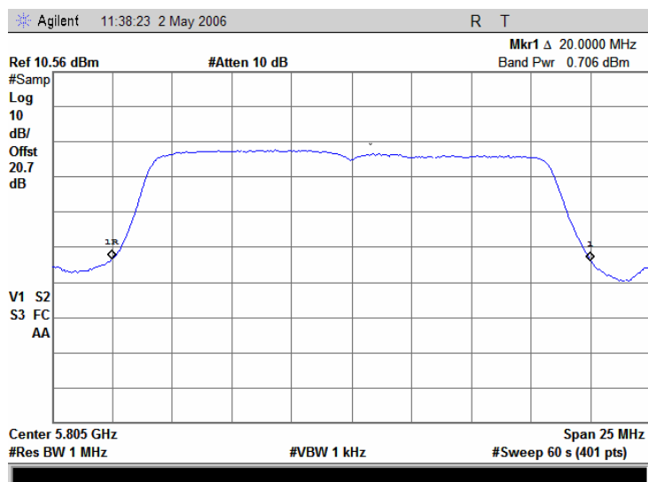
Plot 7.2.7 Peak output power at 5.805 GHz, 6 Mbps
