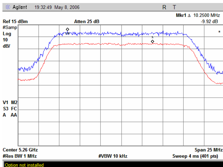
Plot 7.4.8 Peak excursion measurements at 5.260 GHz, 54 Mbps
