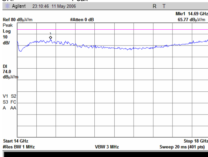
Plot 7.5.52 Radiated emission measurements from 14 to 18 GHz at the 5.26GHz carrier frequency
