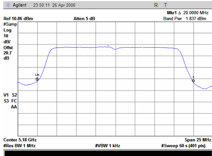
Plot 7.2.2 Peak output power at 5.180 GHz, 6 Mbps
