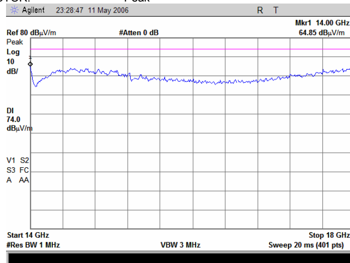
Plot 7.5.106 Radiated emission measurements from 14 to 18 GHz at the 5.785GHz carrier frequency
