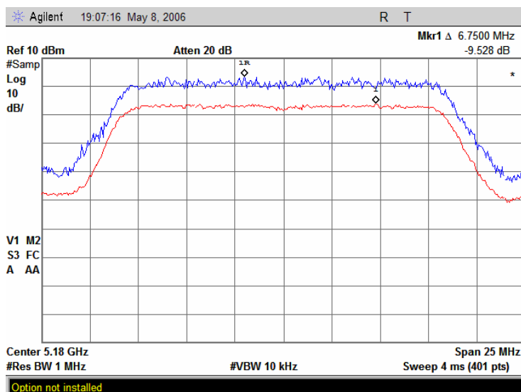
Plot 7.4.7 Peak excursion measurements at 5.180 GHz, 54 Mbps
