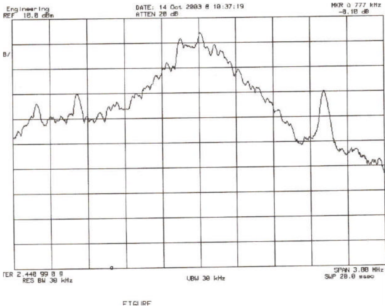
Plot 13: 20 dB BW 2441 MHz
