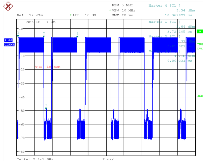
Fig.65 Time of occupancy (Dwell Time): Ch39,Packet 3-DH5
