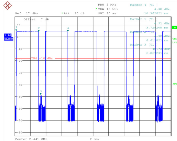
Fig.53 Time of occupancy (Dwell Time): Ch39,Packet DH5
