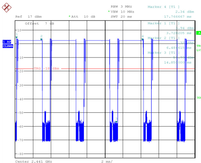
Fig.59 Time of occupancy (Dwell Time): Ch39, Packet 2-DH5
