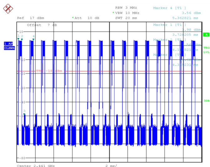
Fig.61 Time of occupancy (Dwell Time): Ch39,Packet 3-DH1
