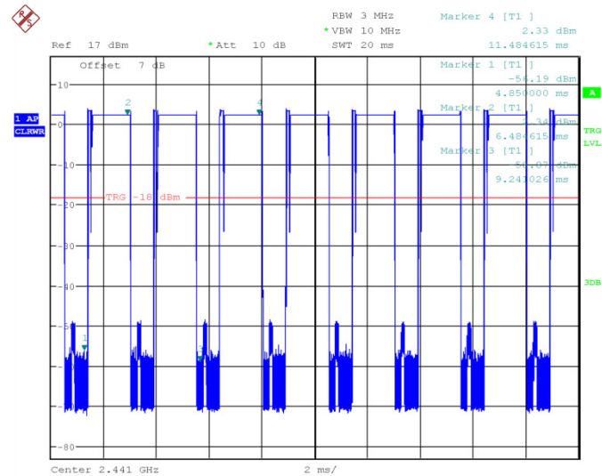
Fig.57 Time of occupancy (Dwell Time): Ch39,Packet 2-DH3
