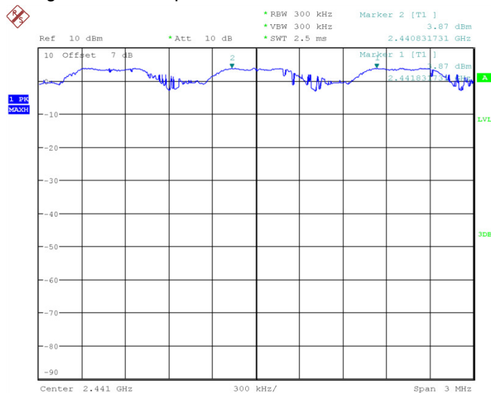
Fig.77 Carrier separation measurement: \pi/4 DQPSK, Ch39
