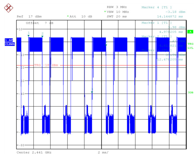
Fig.63 Time of occupancy (Dwell Time): Ch39,Packet 3-DH3
