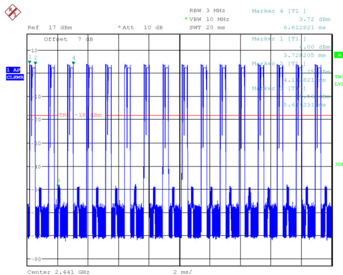
Fig.55 Time of occupancy (Dwell Time): Ch39, Packet 2-DH1
