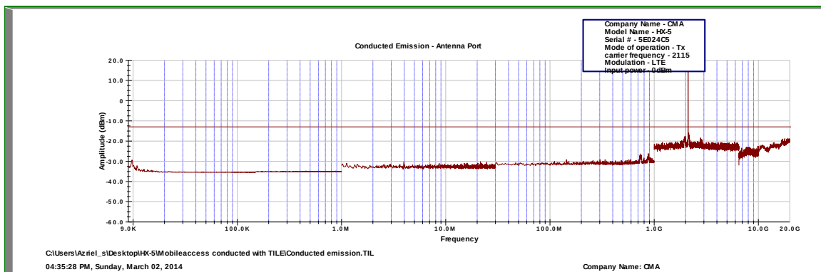
Figure 88.— 2115.00 MHz LTE
