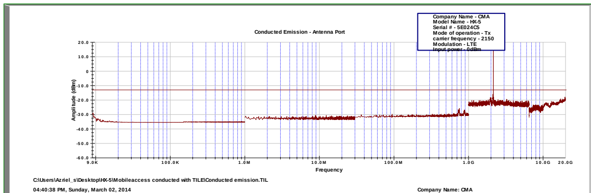
Figure 90.— 2150.00 MHz LTE
