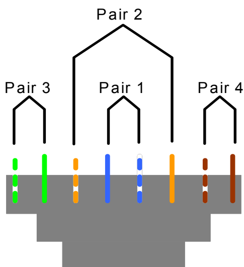
Figure 7 T568A Wiring
