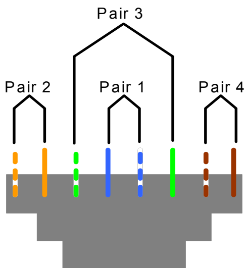
Figure 8 T568B Wiring
