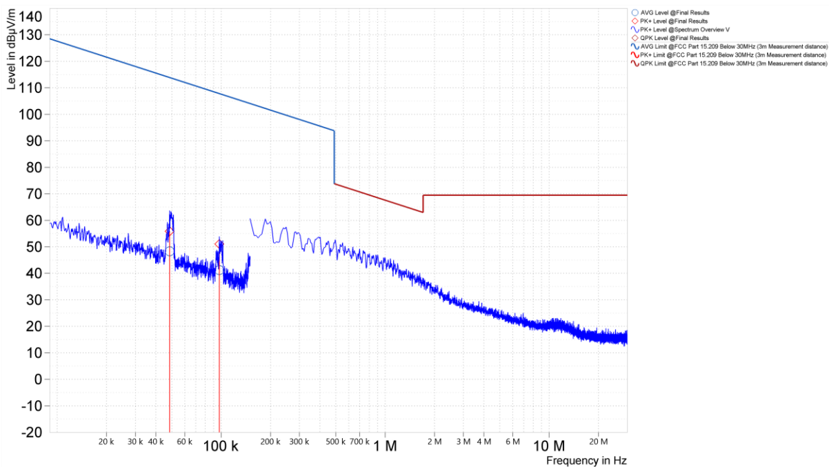
Figure 19. Worst Case Spurious Emissions, 9kHz – 30MHz, 802.11n, Coaxial Loop (Middle Channel)
