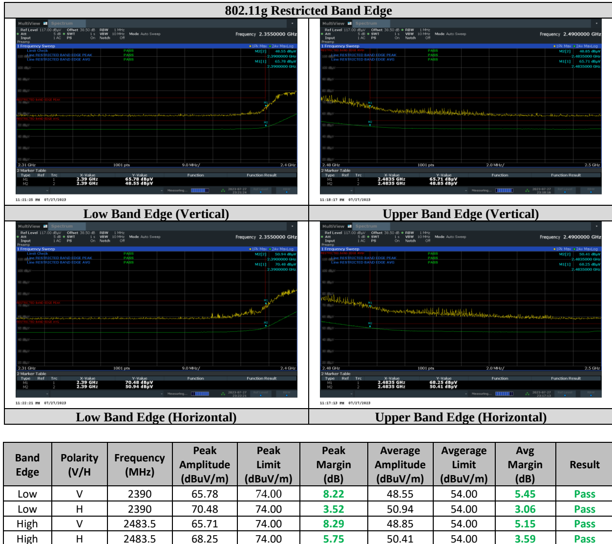
Figure 27. Restricted Band Edge Measurements (802.11g)
