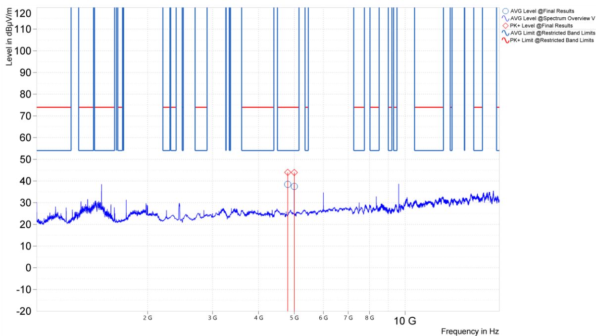
Figure 7. Worst Case Spurious Emissions, 1GHz – 18GHz, 802.11b, Vertical Polarity (Middle Channel)
