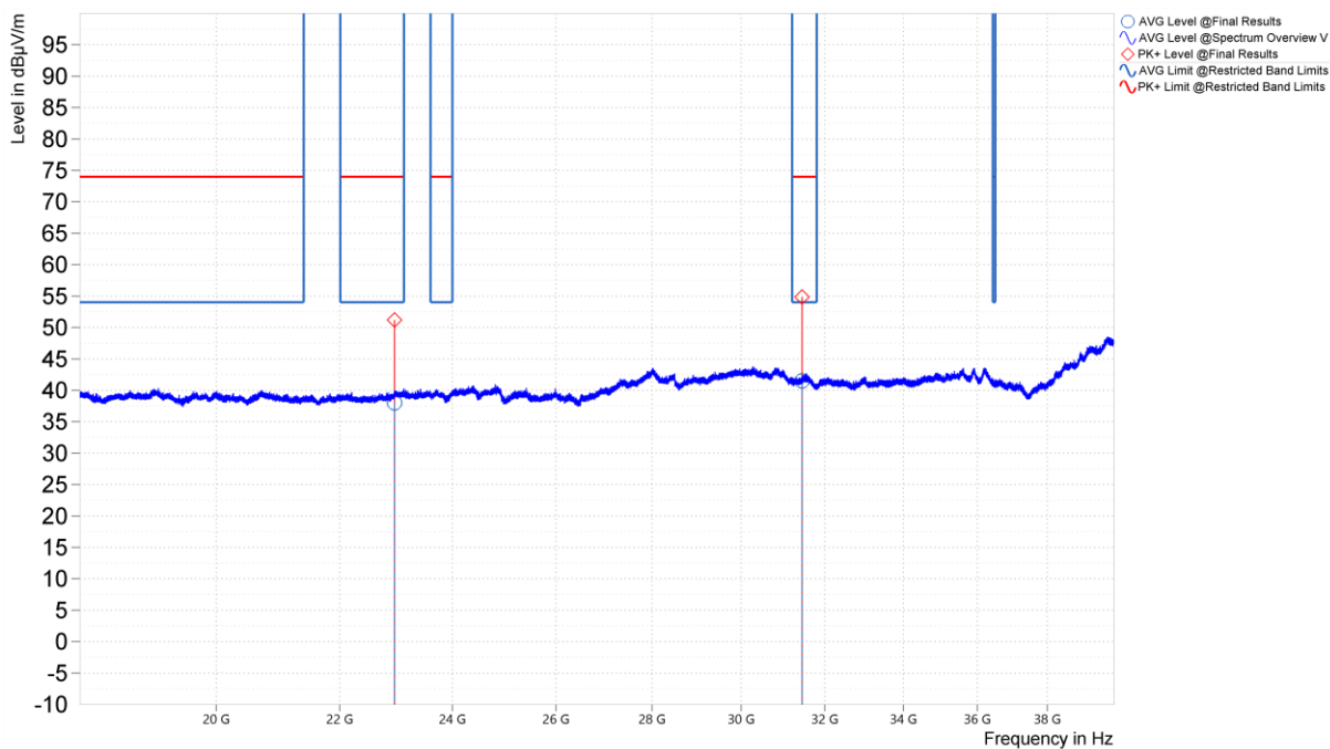
Figure 17. Worst Case Spurious Emissions, 18GHz – 40GHz, 802.11g, Vertical Polarity (Middle Channel)
