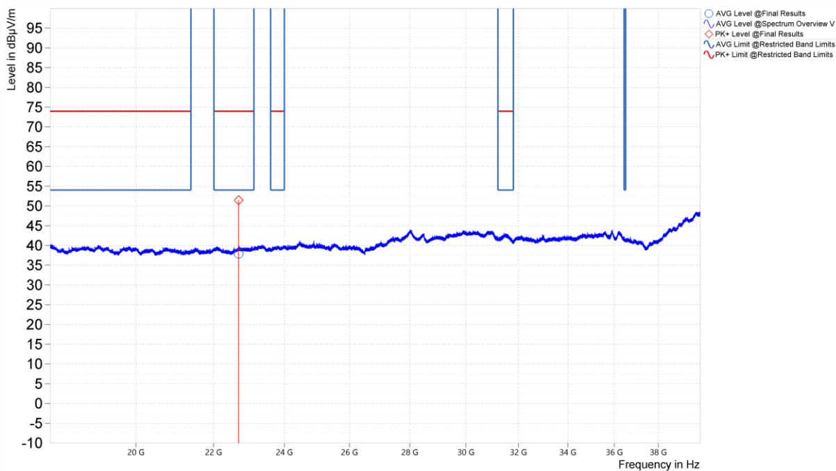
Figure 25. Worst Case Spurious Emissions, 18GHz – 40GHz, 802.11n, Vertical Polarity (Middle Channel)
