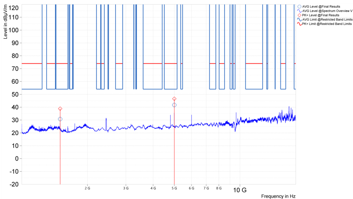
Figure 15. Worst Case Spurious Emissions, 1GHz – 18GHz, 802.11g, Vertical Polarity (Middle Channel)
