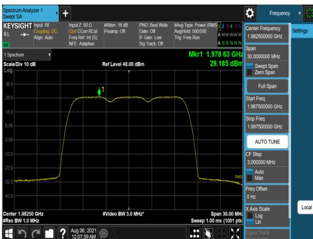
Plot 7-623. Peak Power Spectral Density Plot (B2_5M+5M+5M_3C_16QAM - High Channel, Port 2)
