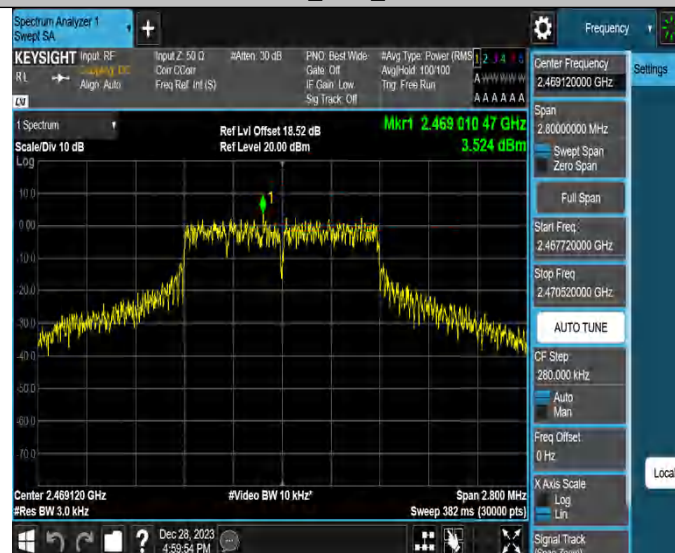
1.4MHz_Ant3_2469.12
