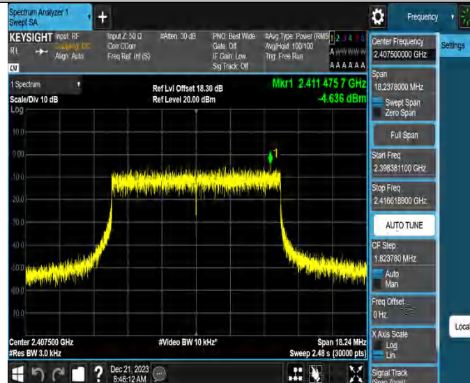
10MHz_Ant3_2407.5
