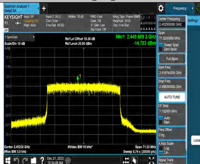
40MHz_Ant3_2452.5
