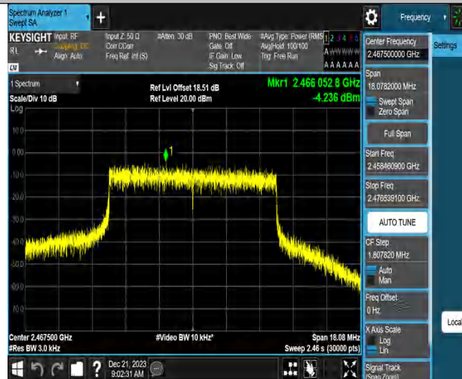
10MHz_Ant3_2467.5
