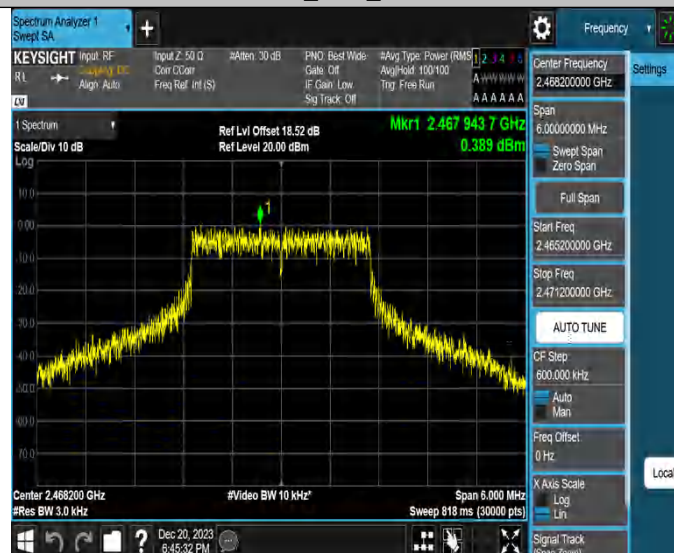
3MHz_Ant3_2468.2
