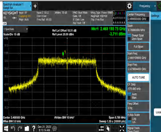
5MHz_Ant3_2469.5
