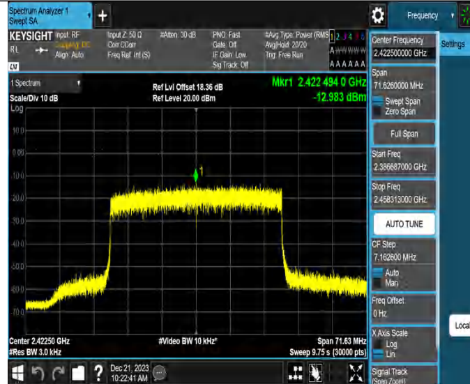
40MHz_Ant3_2422.5
