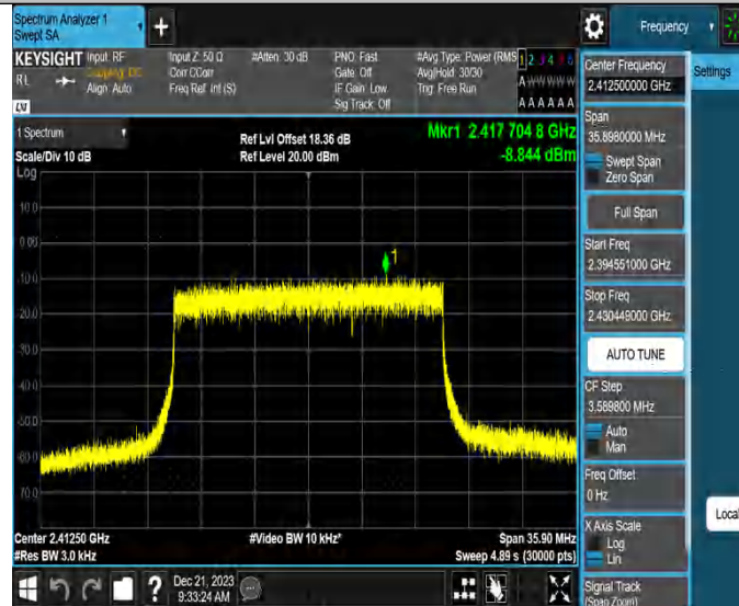
20MHz_Ant3_2412.5
