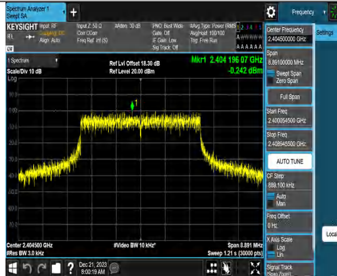
5MHz_Ant3_2404.5
