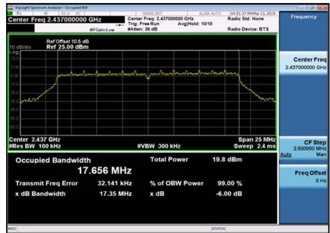
6dB Bandwidth-802.11n(HT20),2437MHz
