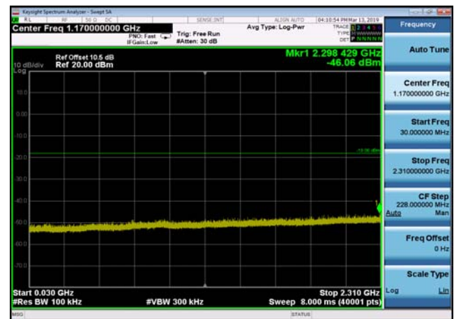
,Plot 3,30MHz~2310MHz-802.11g,2462MHz
