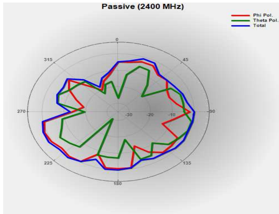
2400 Azimuth 0°
