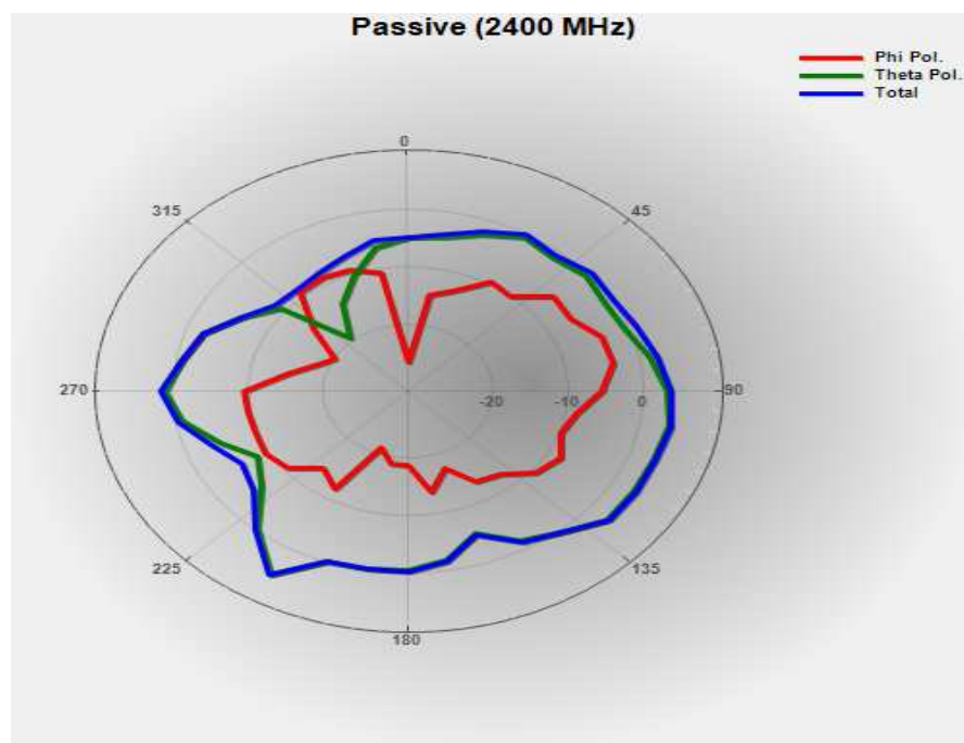
2400 MHz Azimuth 90°
