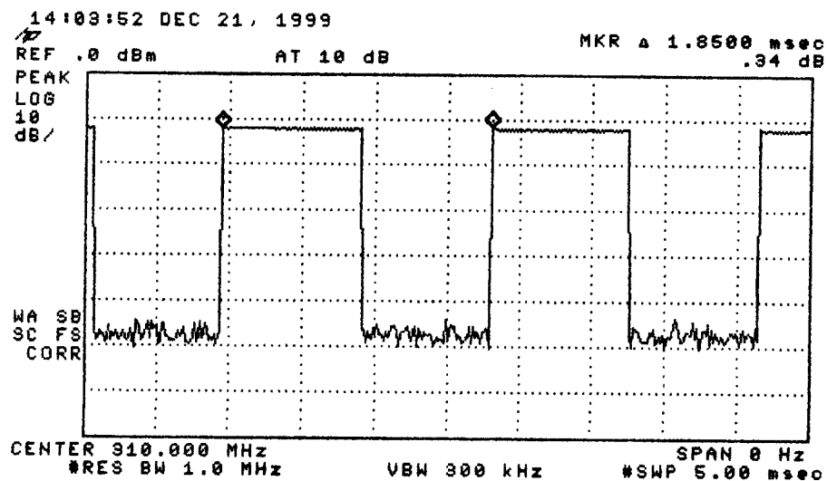
Figure 6.1(b). Transmissions modulation characteristics: (top) pulse width, (bottom) pulse period. (310 MHz, 50% duty factor)
