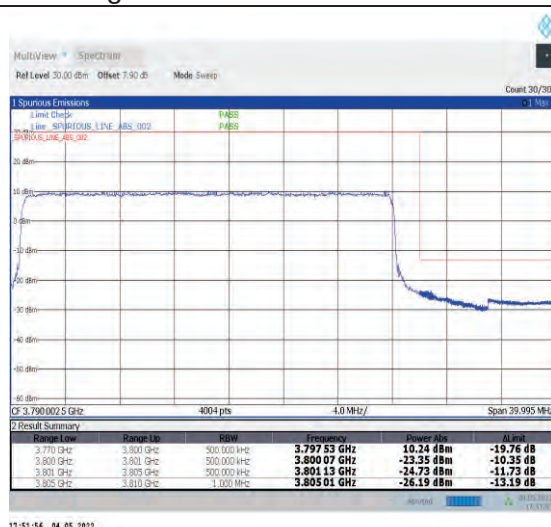
1-N78-3700-3800--30-30-H-3-DFT-PI2BPSK-Outer _Full-75@0-Ant1-PASS-see graph
