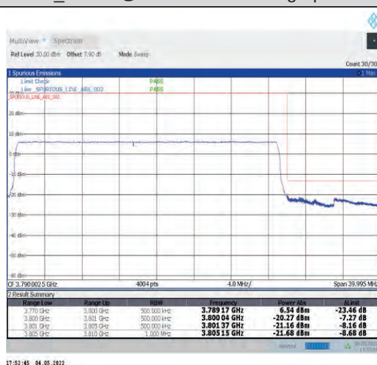
1-N78-3700-3800--30-30-H-6-CP-QPSK-Outer_Fu ll-78@0-Ant1-PASS-see graph
