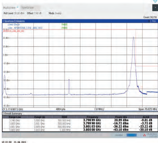
1-N78-3700-3800--30-60-H-5-CP-QPSK-Edge_1RB_Right-1@161-Ant1-PASS-see graph
