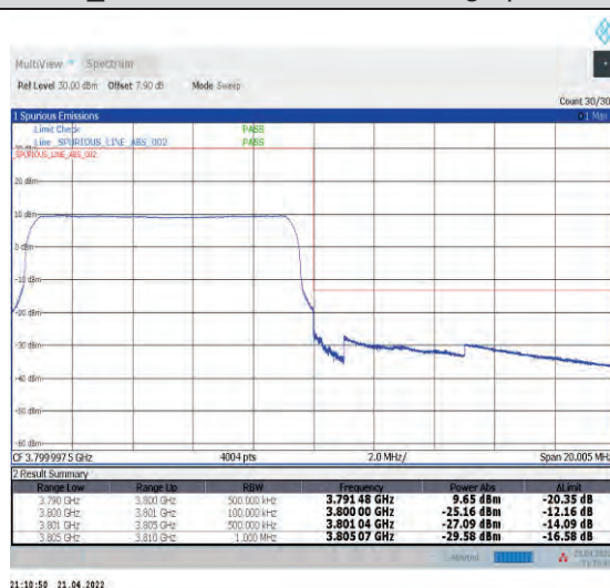
1-N78-3700-3800--30-10-H-6-CP-QPSK-Outer_Fu ll-24@0-Ant1-PASS-see graph
