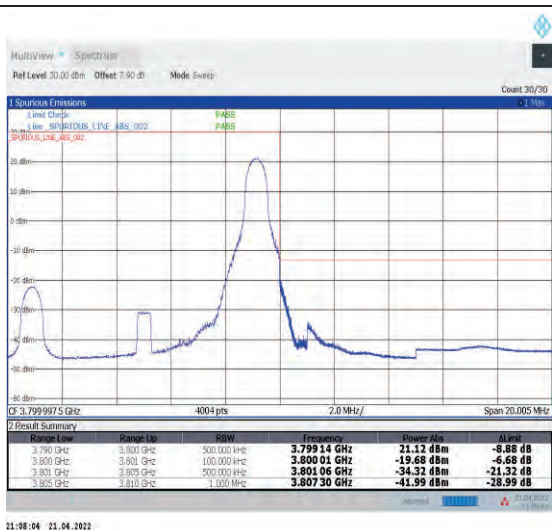
1-N78-3700-3800--30-10-H-2-DFT-PI2BPSK-Edge_1R B_Right-1@23-Ant1-PASS-see graph
