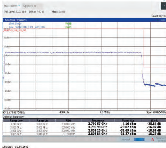
1-N78-3700-3800--30-60-H-3-DFT-PI2BPSK-Outer_Full-162@0-Ant1-PASS-see graph
