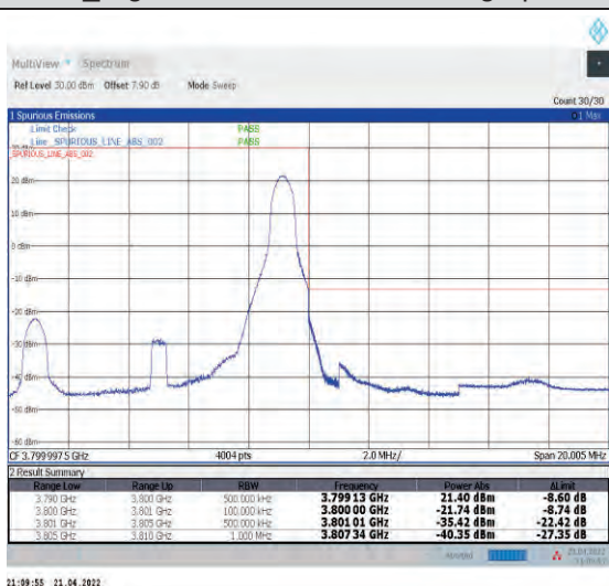
1-N78-3700-3800--30-10-H-5-CP-QPSK-Edge_1RB_R ight-1@23-Ant1-PASS-see graph
