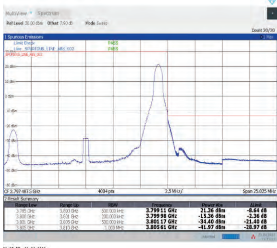
1-N78-3700-3800--30-15-H-5-CP-QPSK-Edge_1RB_R ight-1@37-Ant1-PASS-see graph
