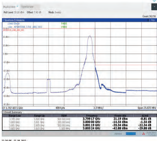
1-N78-3700-3800--30-15-H-2-DFT-PI2BPSK-Edge_1R B_Right-1@37-Ant1-PASS-see graph
