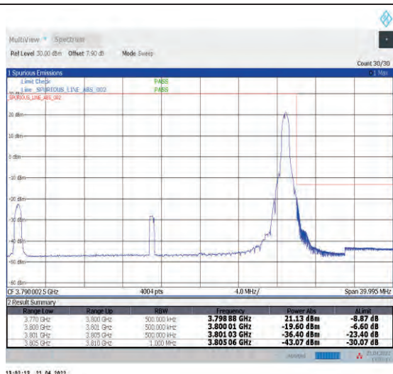
1-N78-3700-3800--30-30-H-2-DFT-PI2BPSK-Edge_1R B_Right-1@77-Ant1-PASS-see graph
