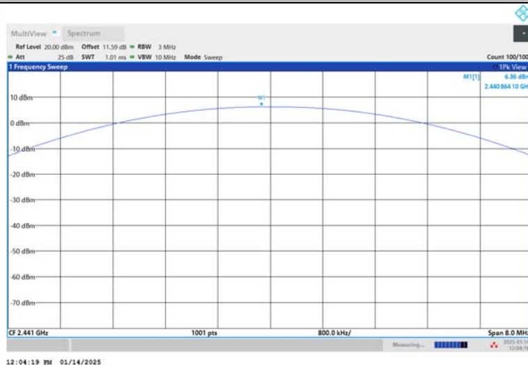
2DH5-Ant1-2441-PASS
