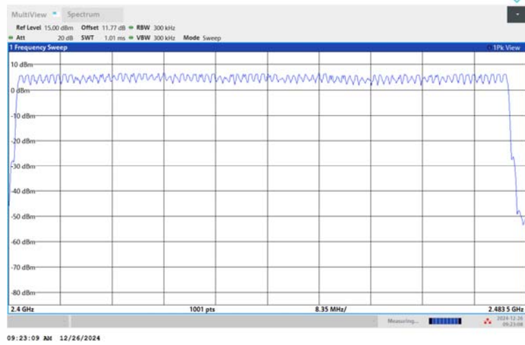
2DH5-Ant1-Hop-PASS
