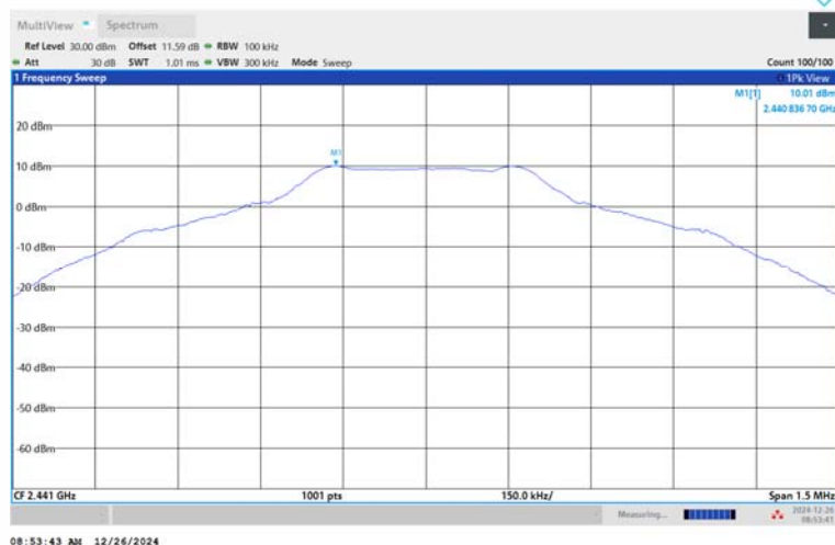
DH5-Ant1-2441-PASS
