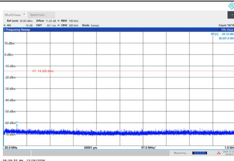
3DH5-Ant1-2480-30~1000-PASS
