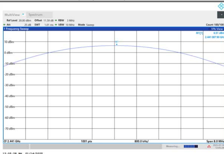
3DH5-Ant1-2441-PASS
