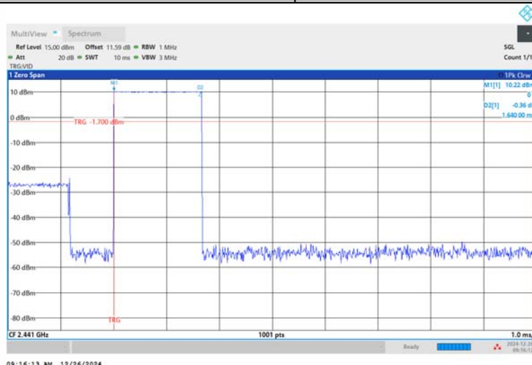
DH3-Ant1-Hop-PASS
