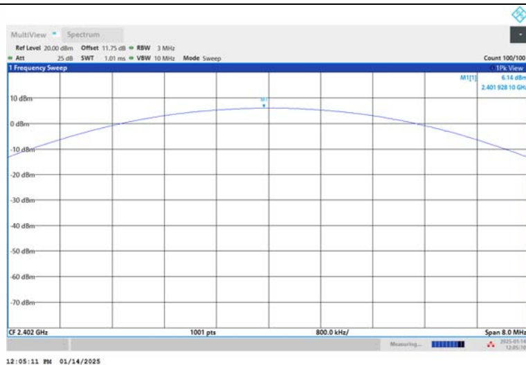
3DH5-Ant1-2402-PASS
