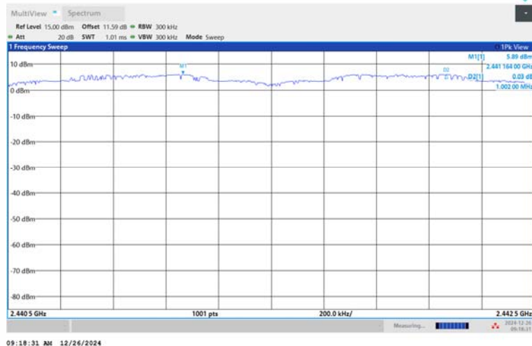
2DH5-Ant1-Hop_2441-PASS
