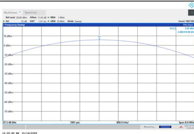
3DH5-Ant1-2480-PASS
