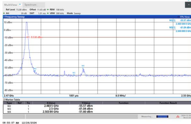
DH5-Ant1-2480-PASS
