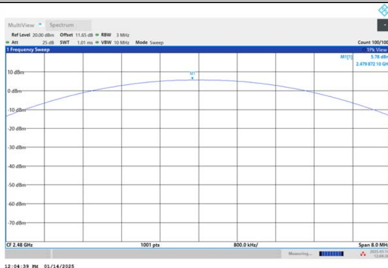
2DH5-Ant1-2480-PASS
