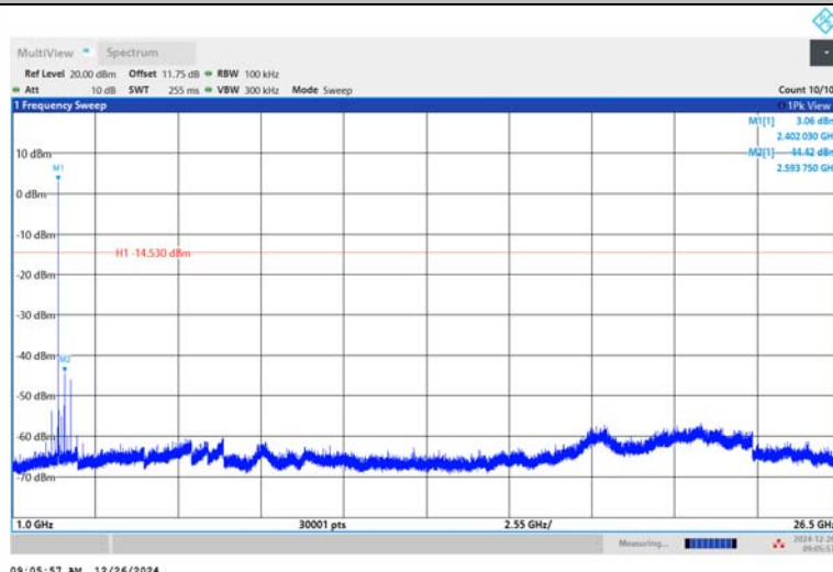
3DH5-Ant1-2402-1000~26500-PASS
