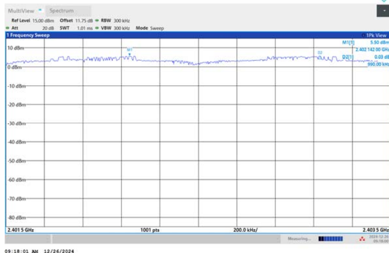
2DH5-Ant1-Hop_2402-PASS
