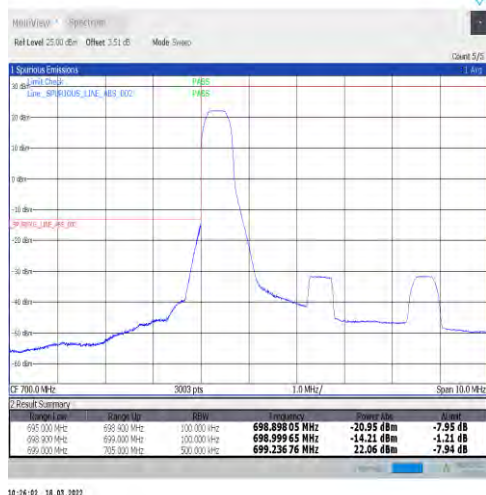
1-N12-15-5-L-1-DFT-PI2BPSK-Edge_1RB_Left-1@0-Ant1-PASS-see graph
