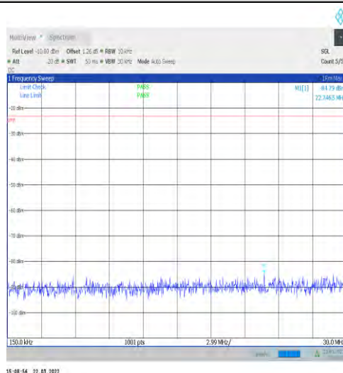
1-N12-15-15-M-1-DFT-PI2BPSK-Inner_1RB_Left-1@ 1-0.15-30-Ant1--84.79--23-PASS
