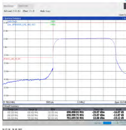
1-N12-15-5-L-6-CP-QPSK-Outer_Full-25@0-Ant1-PASS-see graph
