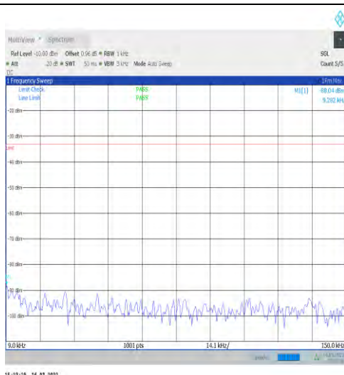
1-N12-15-15-H-1-DFT-PI2BPSK-Inner_1RB_Left-1 @1-0.009-0.15-Ant1--88.04--33-PASS
