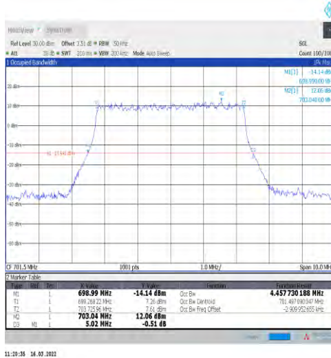
1-N12-15-5-L-3-DFT-16QAM-Outer_Full-25@0-Ant1-4 4.458-5.020-≤5-PASS
