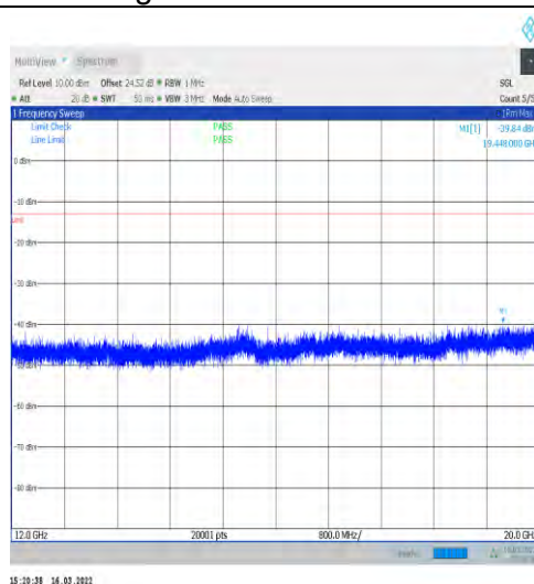
1-N12-15-15-L-1-DFT-PI2BPSK-Inner_1RB_Left-1@ 1-12000-20000-Ant1--39.84--13-PASS
