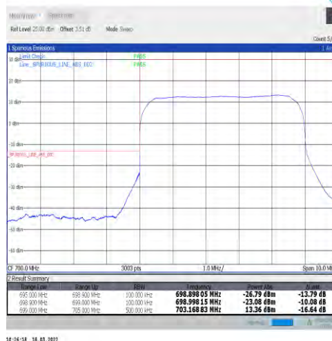
1-N12-15-5-L-3-DFT-PI2BPSK-Outer_Full-25@0-Ant1-PASS-see graph
