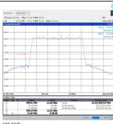
1-N12-15-15-H-4-DFT-64QAM-Outer_Full-75@0-Ant1 1-13.422-14.460≤15-PASS
