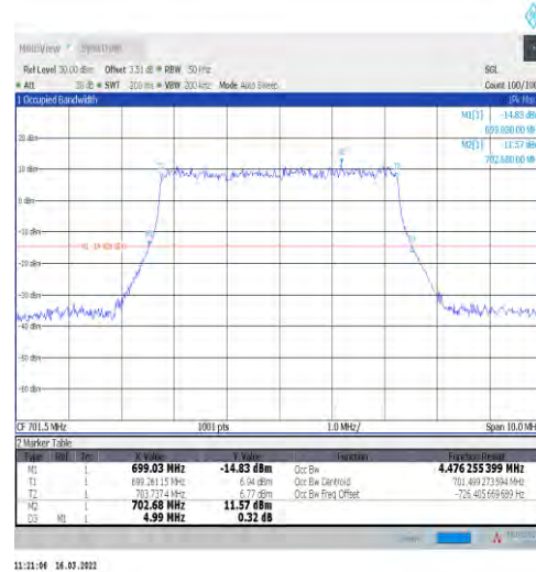
1-N12-15-5-L-4-DFT-64QAM-Outer_Full-25@0-Ant1-4 -4.476-4.990-≤5-PASS
