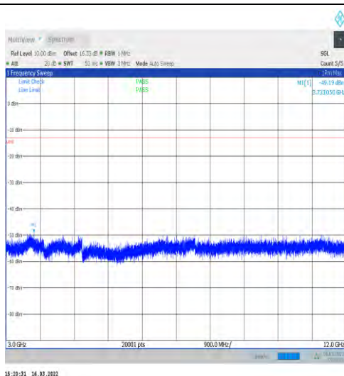
1-N12-15-15-L-1-DFT-PI2BPSK-Inner_1RB_Left-1@ 1-3000-12000-Ant1--49.19--13-PASS
