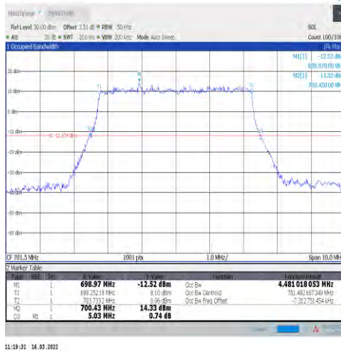
1-N12-15-5-L-1-DFT-QPSK-Outer_Full-25@0-Ant1-4 .481-5.030-≤5-PASS
