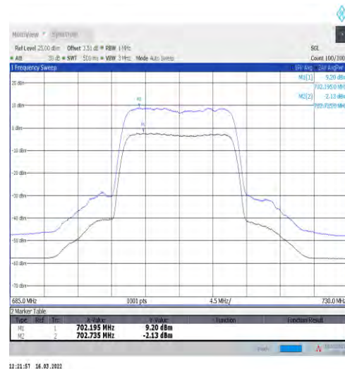
1-N12-15-15-M-2-CP-256QAM-Outer_Full-79@0-Ant t1-11.33-100%-0.00-11.33-PASS-≤13
