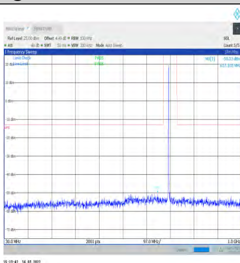
1-N12-15-15-H-1-DFT-PI2BPSK-Inner_1RB_Left-1 @1-30-1000-Ant1--50.33--13-PASS
