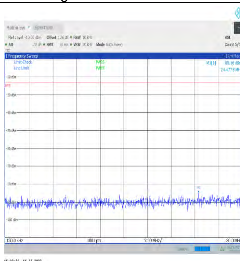
1-N12-15-15-H-1-DFT-PI2BPSK-Inner_1RB_Left-1@ 1-0.15-30-Ant1--85.16--23-PASS
