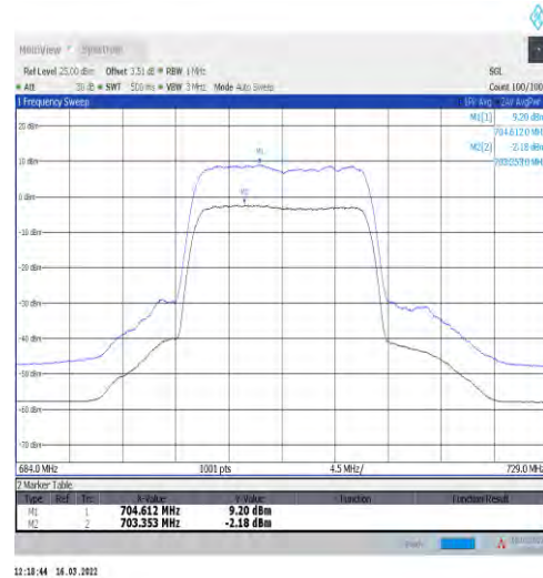
1-N12-15-15-L-2-CP-256QAM-Outer_Full-79@0-Ant 1-11.38-100%-0.00-11.38-PASS-≤13
