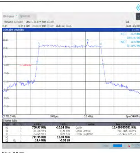
1-N12-15-15-H-1-DFT-QPSK-Outer_Full-75@0-Ant1 -13.451-14.400≤15-PASS
