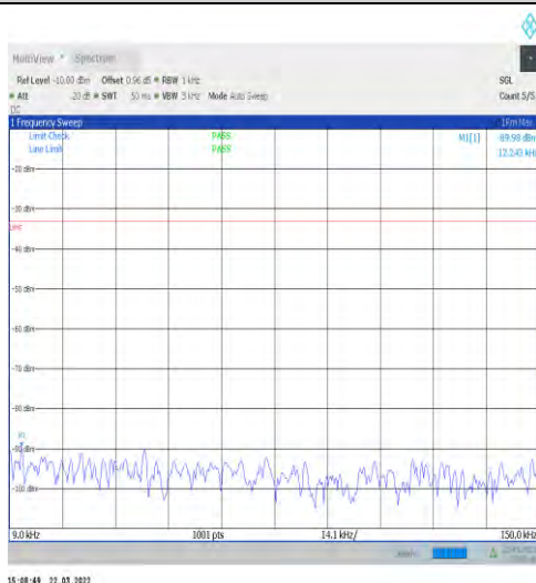
1-N12-15-15-M-1-DFT-PI2BPSK-Inner_1RB_Left-1@ 1-0.009-0.15-Ant1--89.98--33-PASS
