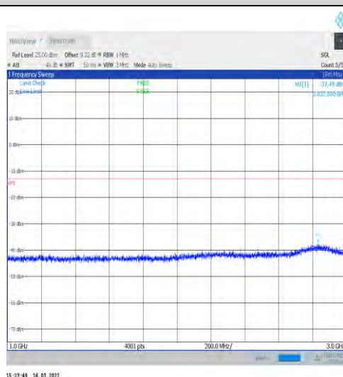
1-N12-15-15-H-1-DFT-PI2BPSK-Inner_1RB_Left-1@ 1-1000-3000-Ant1--37.49--13-PASS
