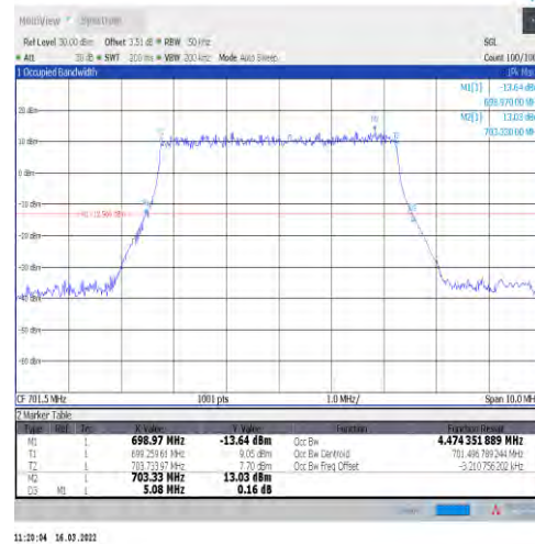
1-N12-15-5-L-2-DFT-PI2BPSK-Outer_Full-25@0-Ant1-4 1-4.474-5.080-≤5-PASS
