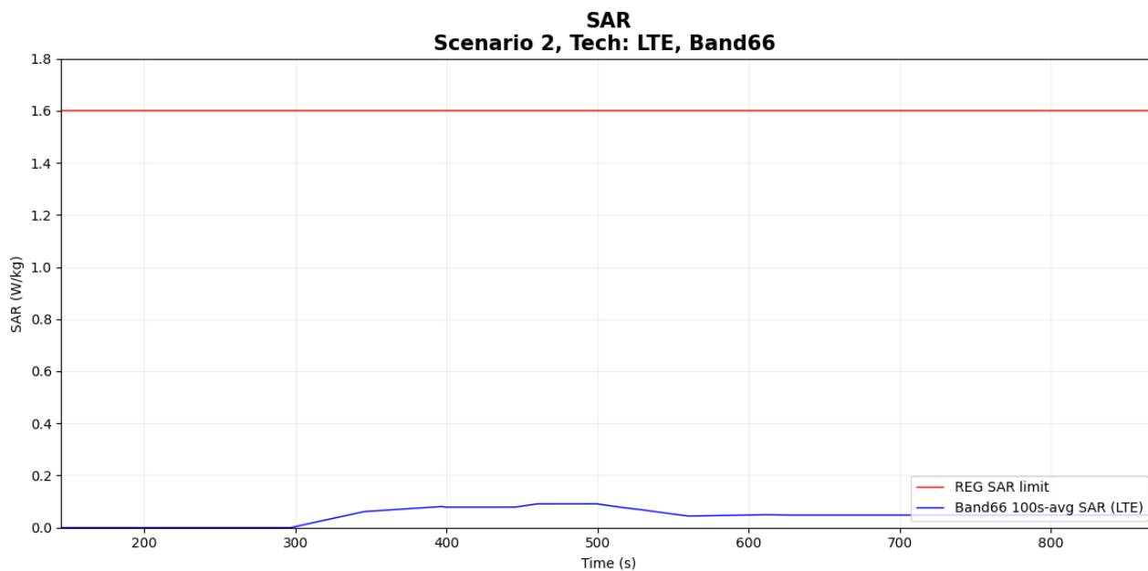
Figure 7-10 Time-averaged SAR
