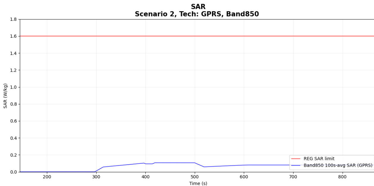
Figure 7-2 Time-averaged SAR
