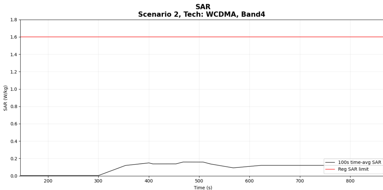
figure 6- 16 Time-averaged SAR
