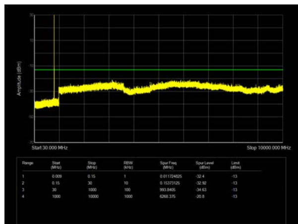
LTE Band 26 3MHz CH Low 30MHz~10GHz
