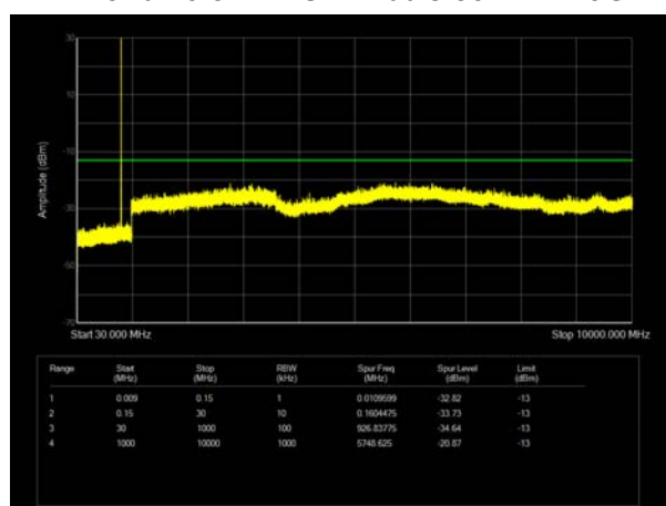
LTE Band 26 3MHz CH Middle 30MHz~10GHz
