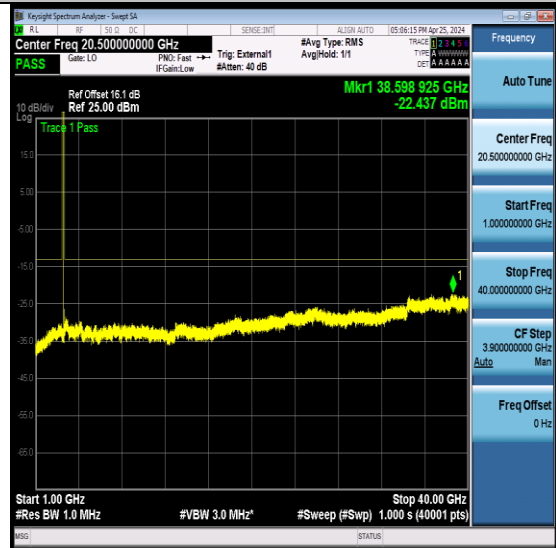
NTNV-N78-3450-3550-PC2-30-20-H-CP-QPSK- Edge_1RB_Left-Ant1-PASS
