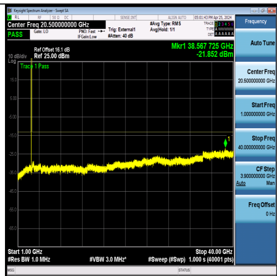
NTNV-N78-3450-3550-PC2-30-20-L-CP-QPSK- Edge_1RB_Left-Ant1-PASS
