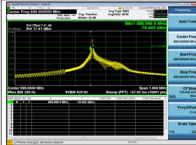
BPSK Low channel-1@0
