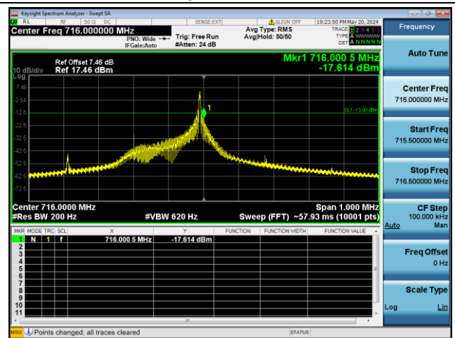
BPSK High channel-1@max
