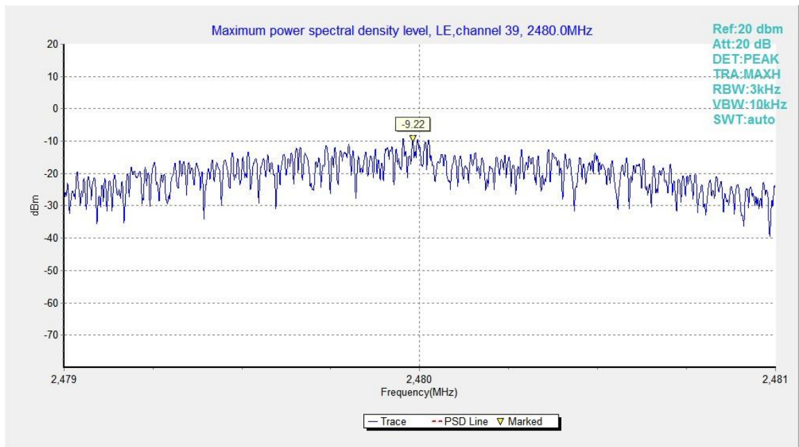
Fig.23. Maximum Power Spectral Density Level Function: GFSK, 2480 MHz
