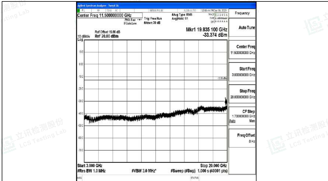
Band2_15MHz_QPSK_18675_1RB#0_3000~20000_3000~20000
