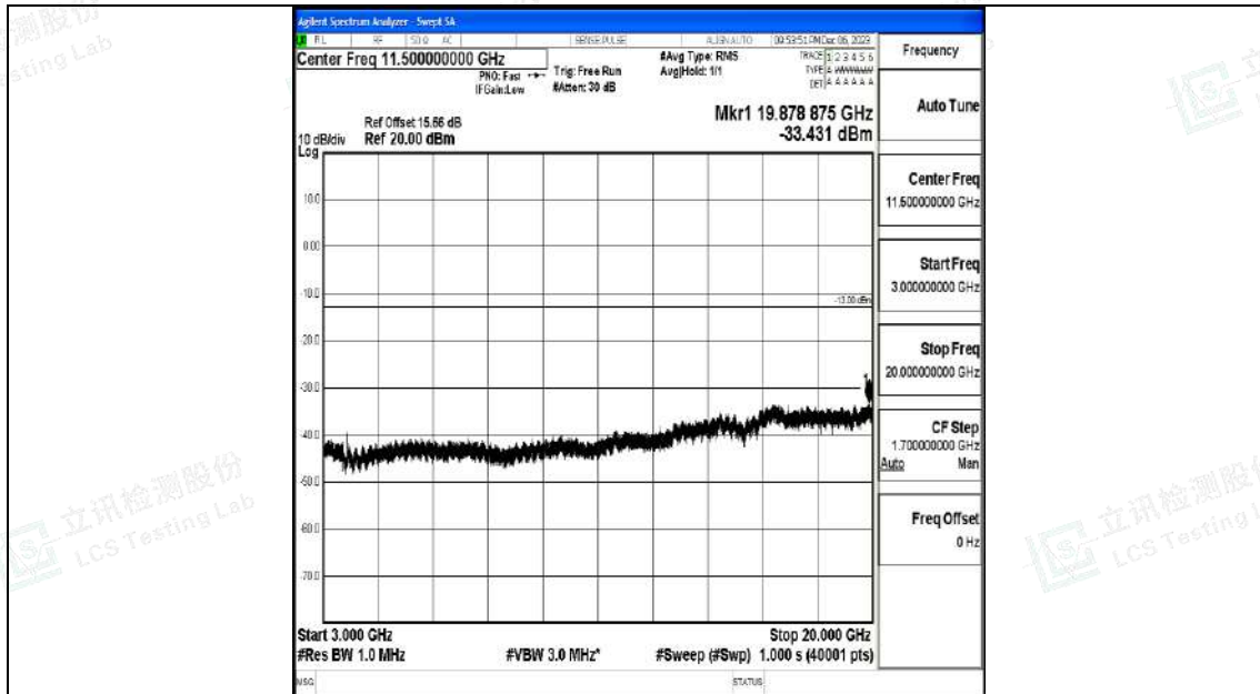
Band2_10MHz_QPSK_18900_1RB#0_3000~20000_3000~20000
