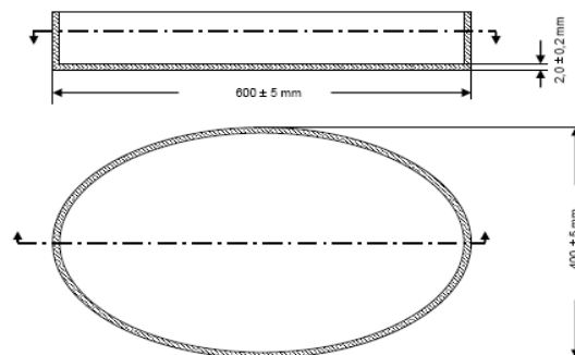
Figure 1: Proportions and shape of Phantom shell
