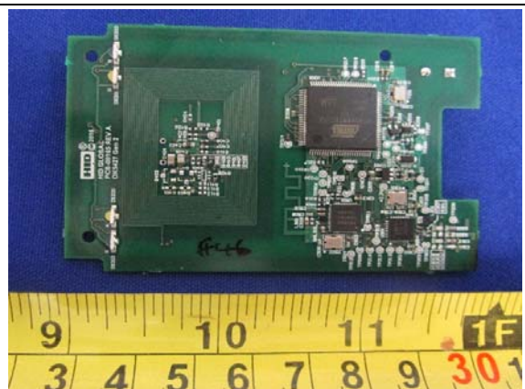
EUT Main PCB - Top View
