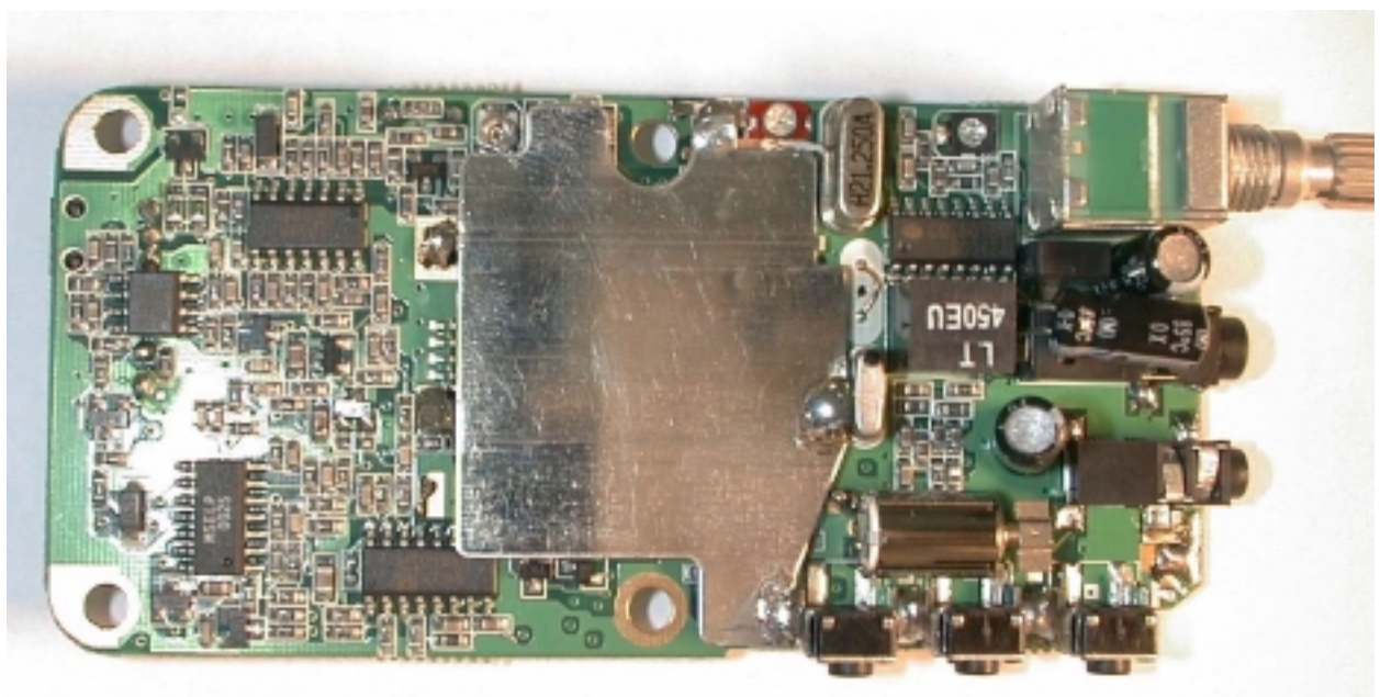
Bottom PCB w/shield
