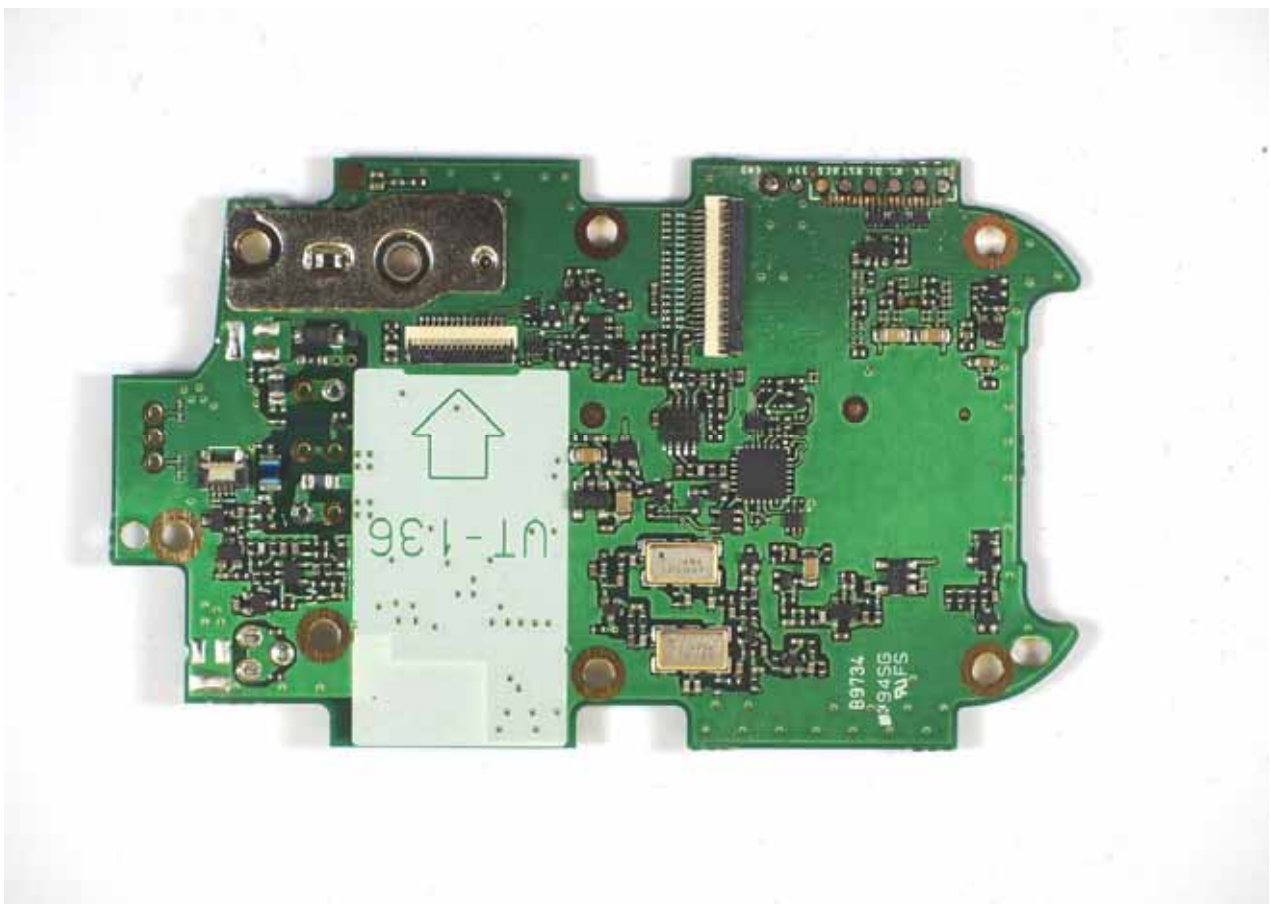
MAIN SIDE A (WITHOUT UT-136)
