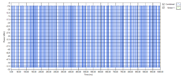
BLE/GFSK 1 Mbps Low Channel, 2402 MHz
