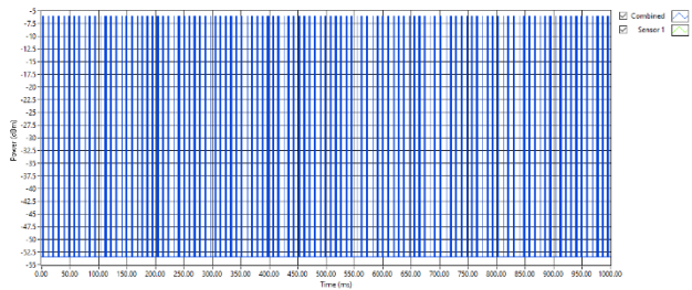
BLE/GFSK 1 Mbps Mid Channel, 2442 MHz
