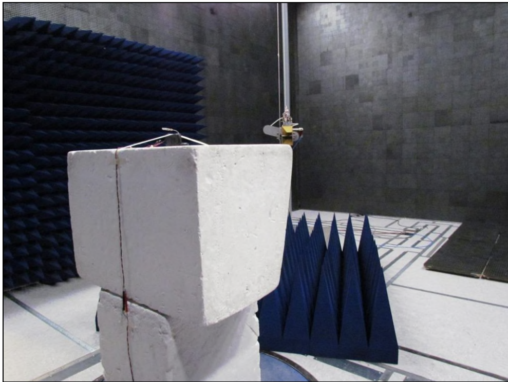
Figure 4: Equipment Under Test – Radiated Emissions – 1-18GHz
