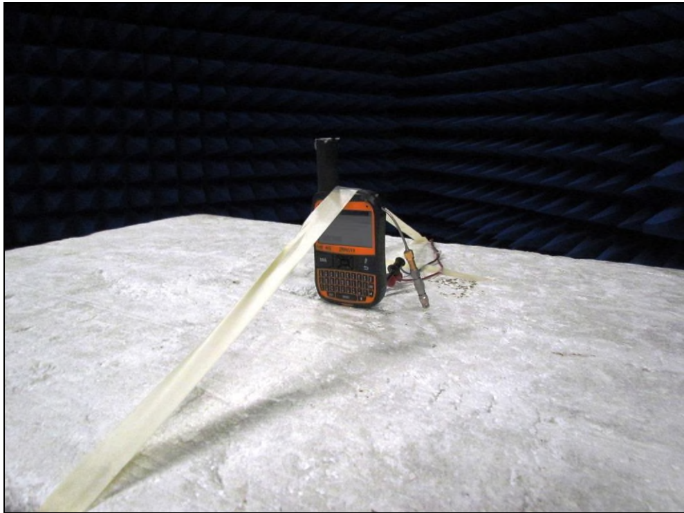
Figure 7: Equipment Under Test – Radiated Emissions – Z-orientation
