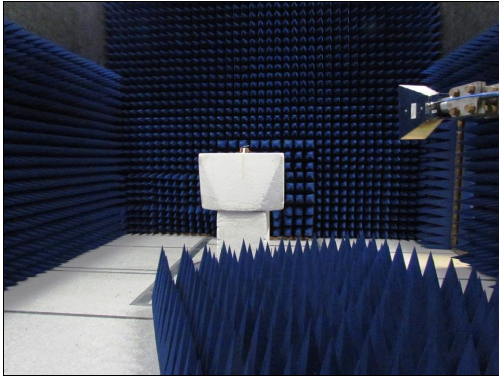
Figure 3: Equipment Under Test – Radiated Emissions – 1-18GHz
