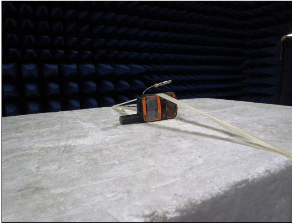
Figure 5: Equipment Under Test – Radiated Emissions – X-orientation
