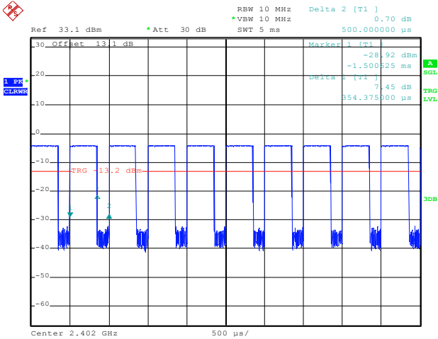
BLE_BT4.0_Ant1_2402
