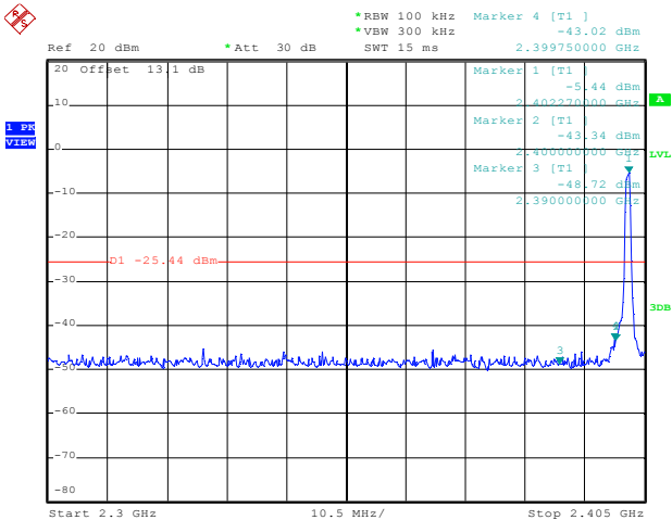
BLE_BT4.0_Ant1_Low_2402
