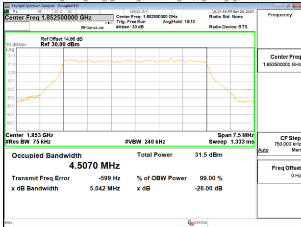
Band25_5MHz_DFT_s_OFDM_SCS15kHz_BPSK_RB25_0_CH376500
