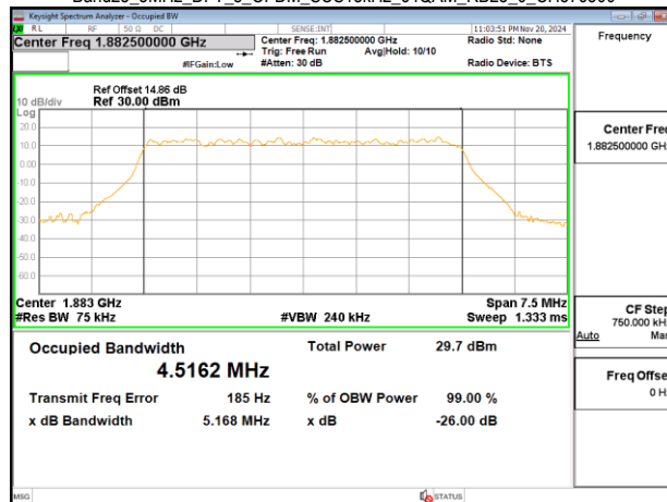
Band25_5MHz_DFT_s_OFDM_SCS15kHz_64QAM_RB25_0_CH376500
