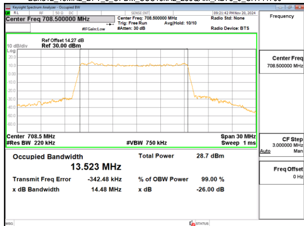
Band12_15MHz_DFT_s_OFDM_SCS15kHz_256QAM_RB75_0_CH141700
