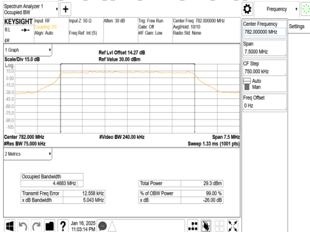
Band13_5MHz_DFT_s_OFDM_SCS15kHz_64QAM_RB25_0_CH156900
