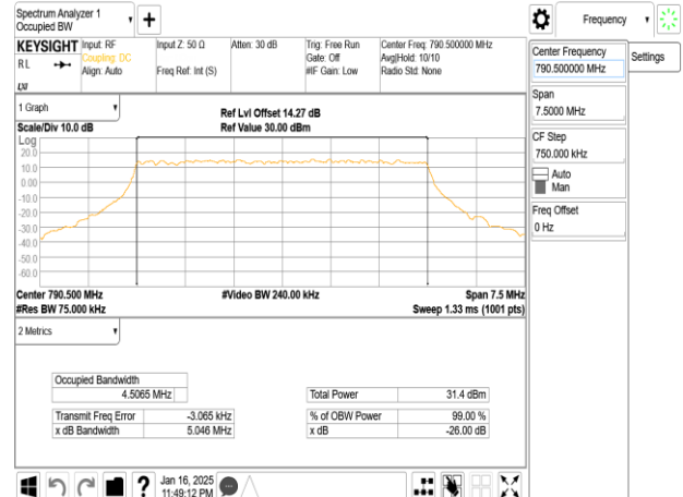
Band14_5MHz_DFT_s_OFDM_SCS15kHz_BPSK_RB25_0_CH158100
