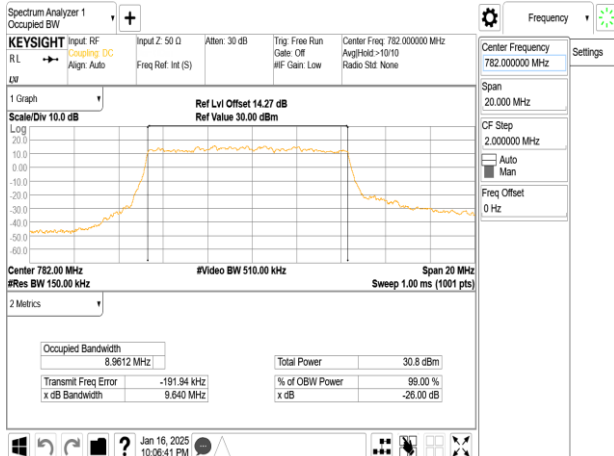
Band13_10MHz_DFT_s_OFDM_SCS15kHz_16QAM_RB50_0_CH156400
