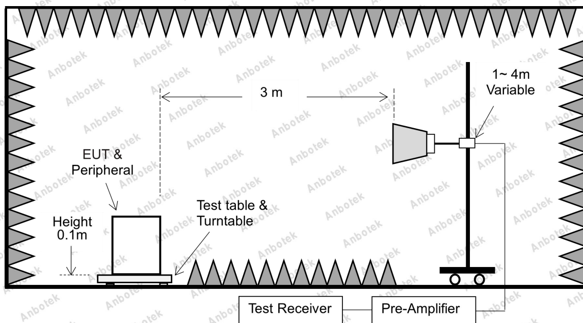
Figure 3. Above 1 GHz
